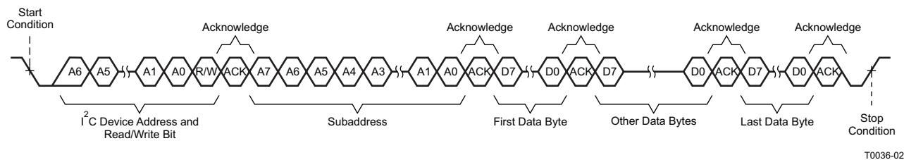
Figure 24. Multiple-Byte Write Transfer
