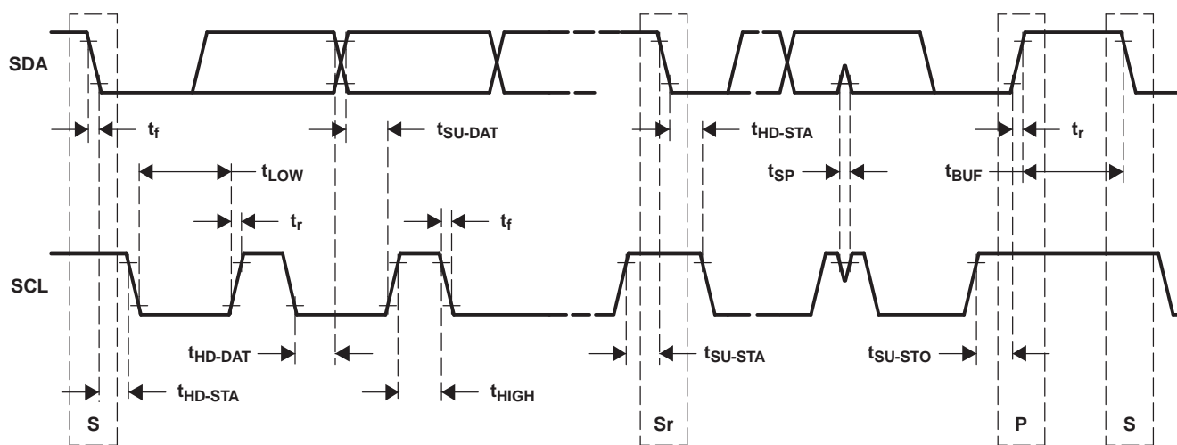
Figure 3. Start and Stop Conditions Timing Waveforms
