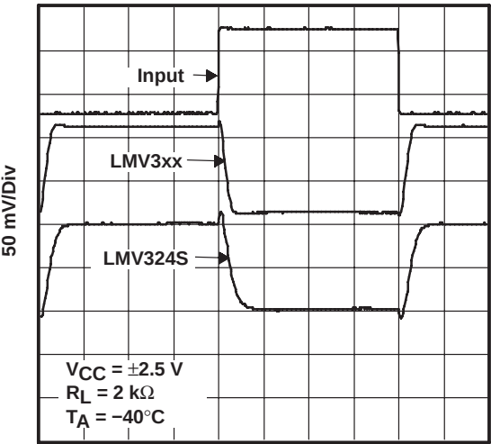
1 μs/Div Figure 38
