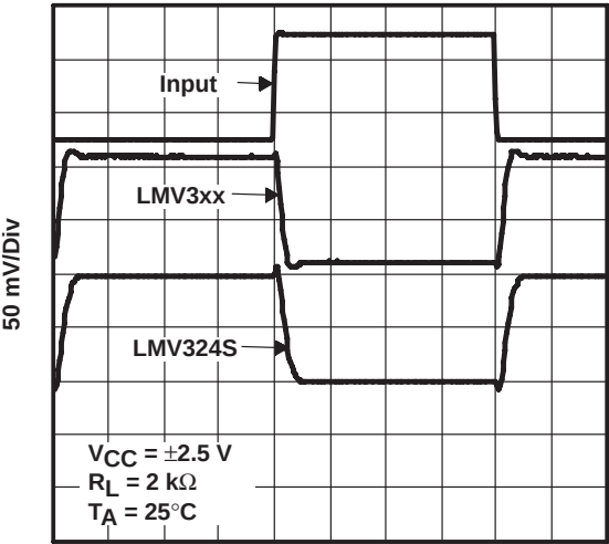
1 μs/Div Figure 36
