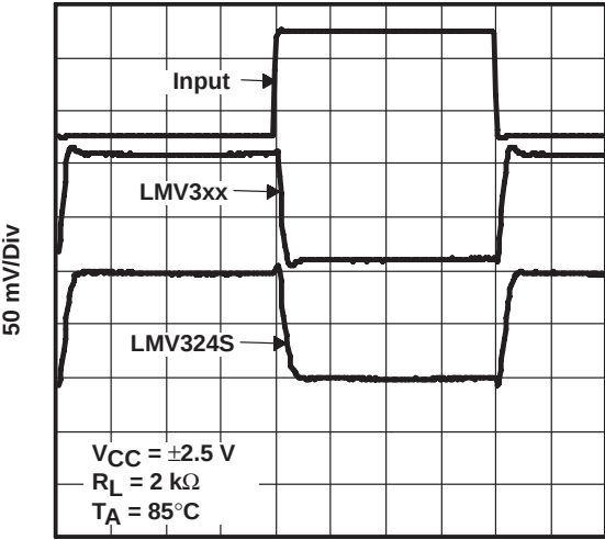
1 μs/Div Figure 37
