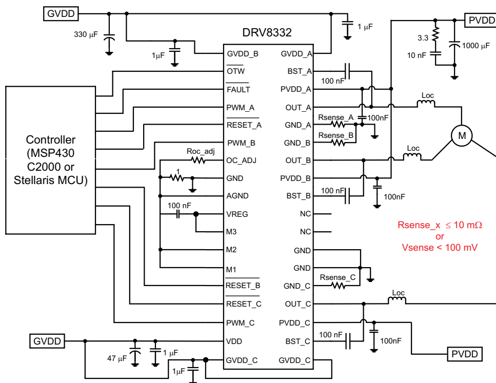
Figure 8. DRV8332 Application Diagram for Three-Phase Operation
