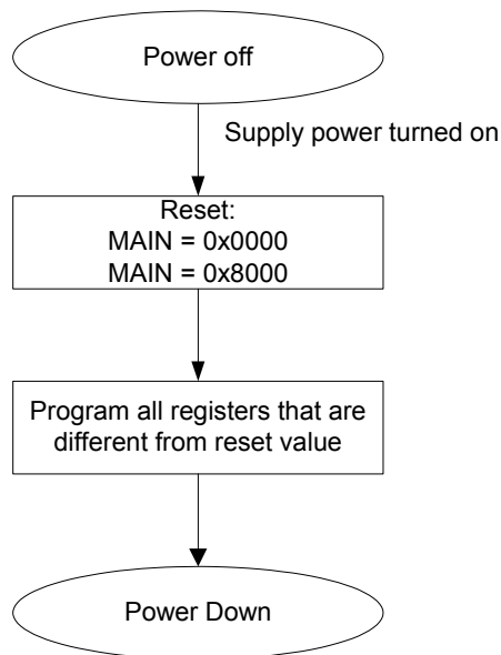
Figure 16. Initializing sequence
