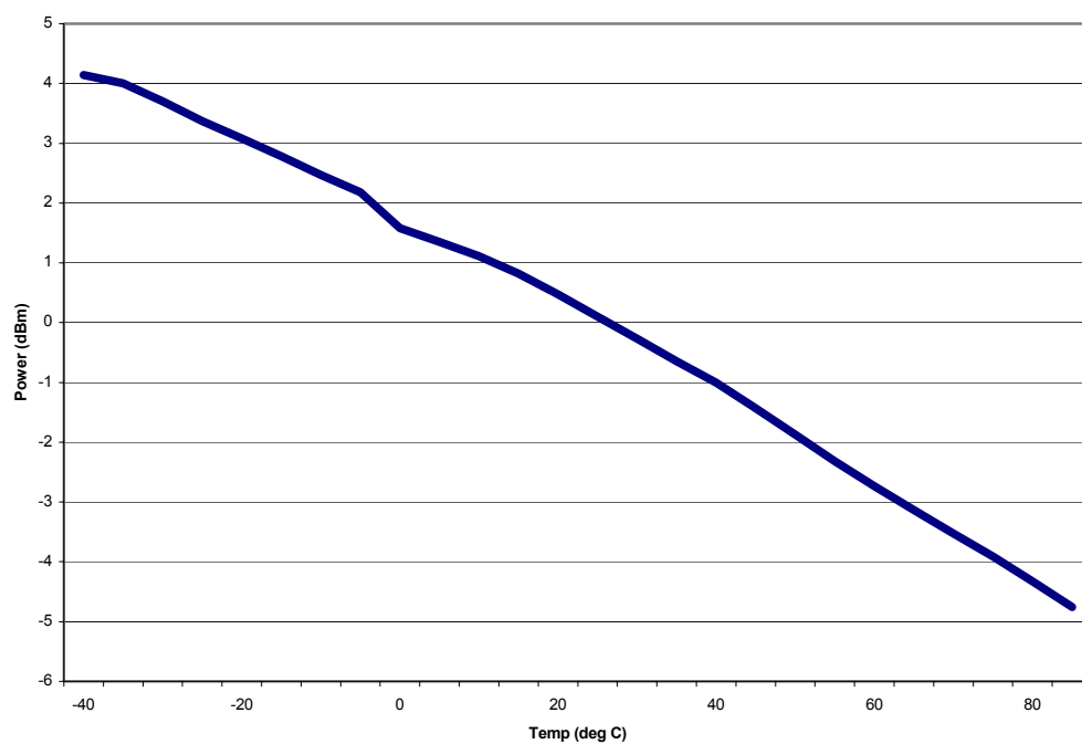
Figure 26 Typical output power vs. temperature
