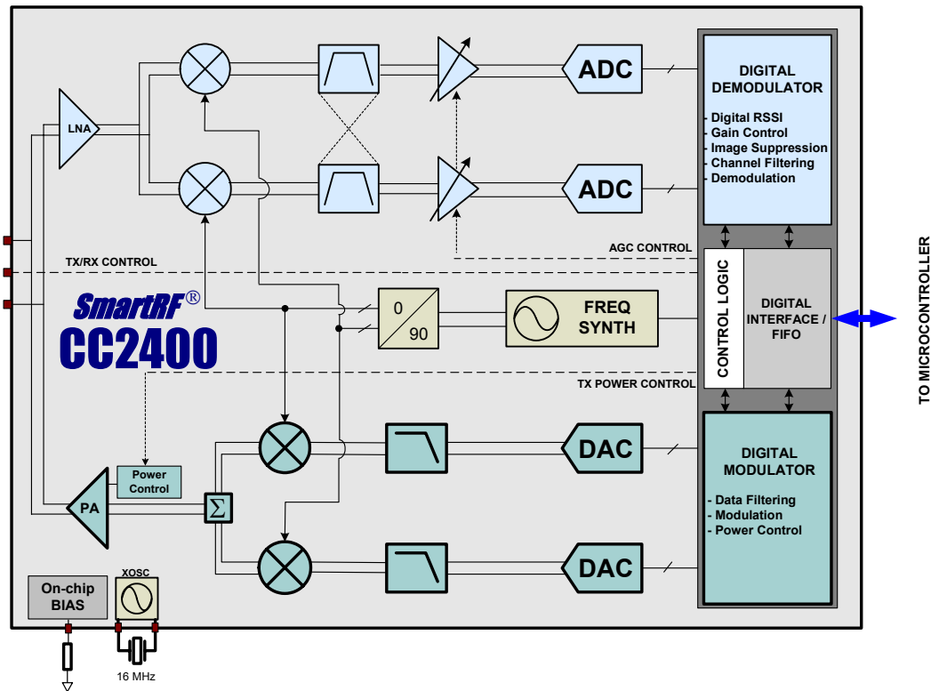
Figure 2. CC2400 simplified block diagram
