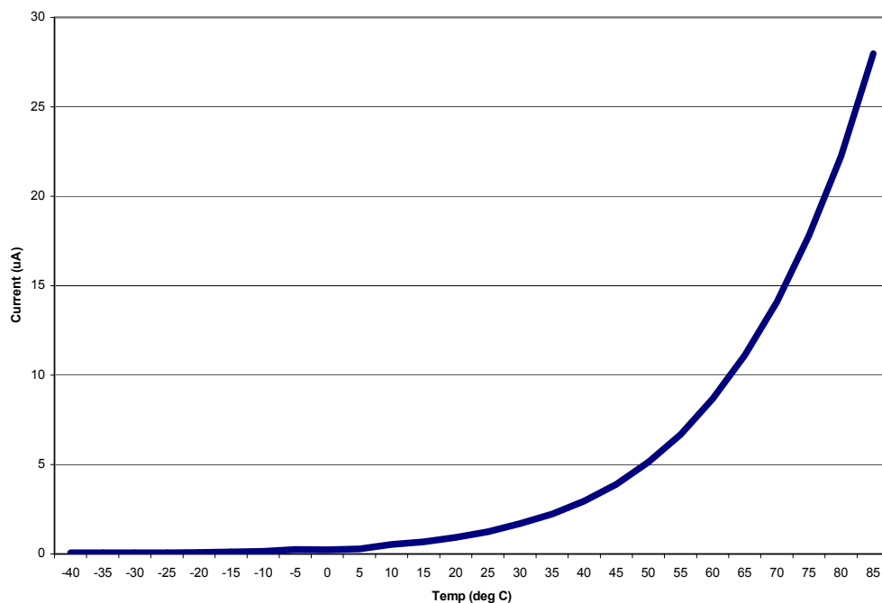
Figure 25 Typical power-down current vs. temperature
