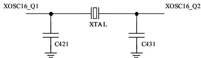
Figure 23. Crystal oscillator circuit
