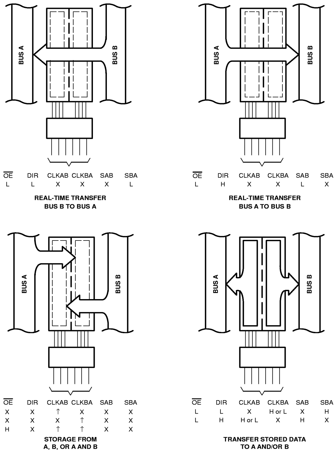
Figure 1. Bus-Management Functions
