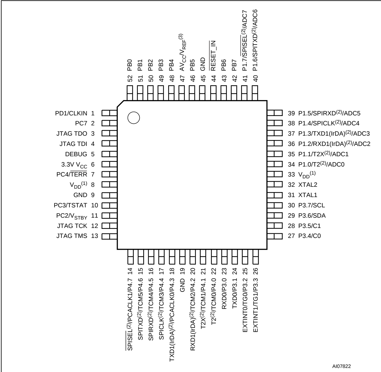
Figure 3. TQFP52 Connections
