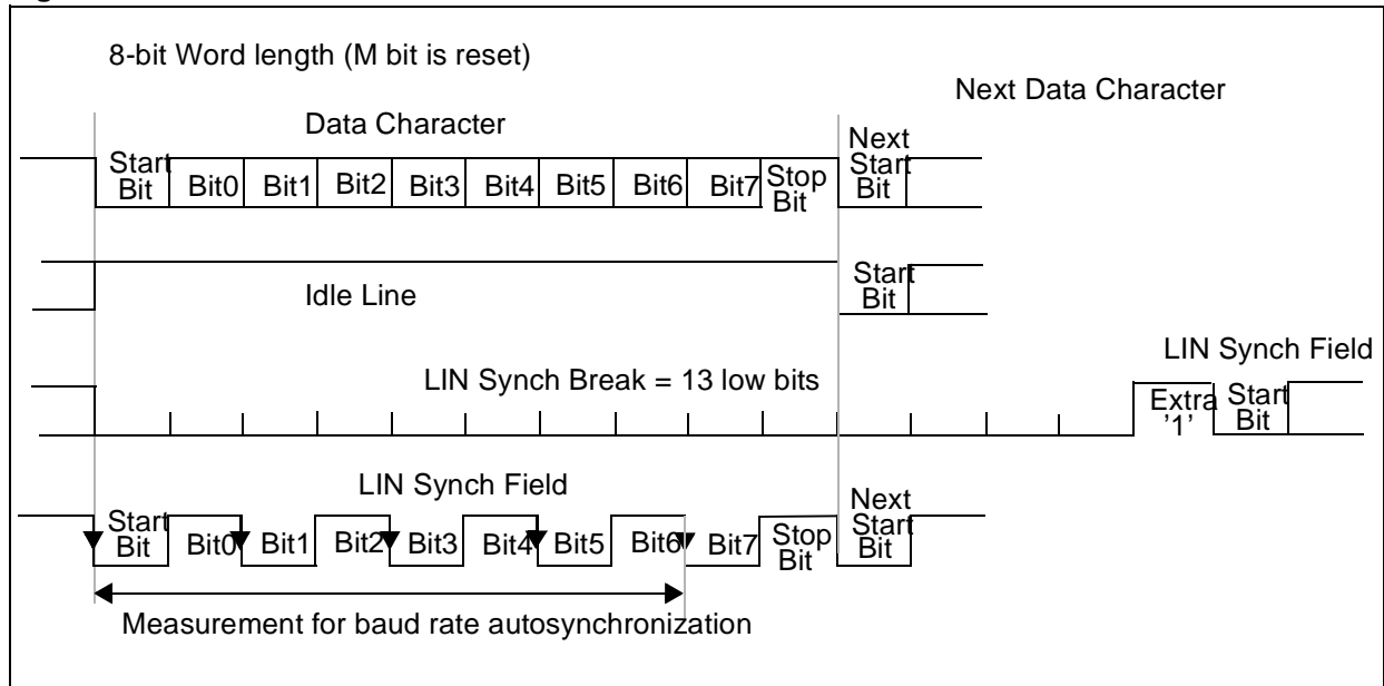
Figure 63. LIN characters
