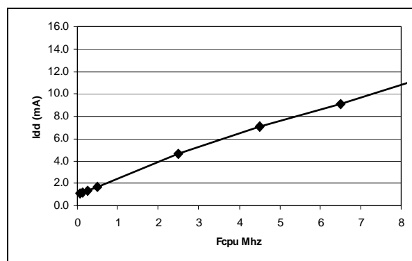
Figure 129. Typical I_{DD} in RUN vs. f_{CPU}
