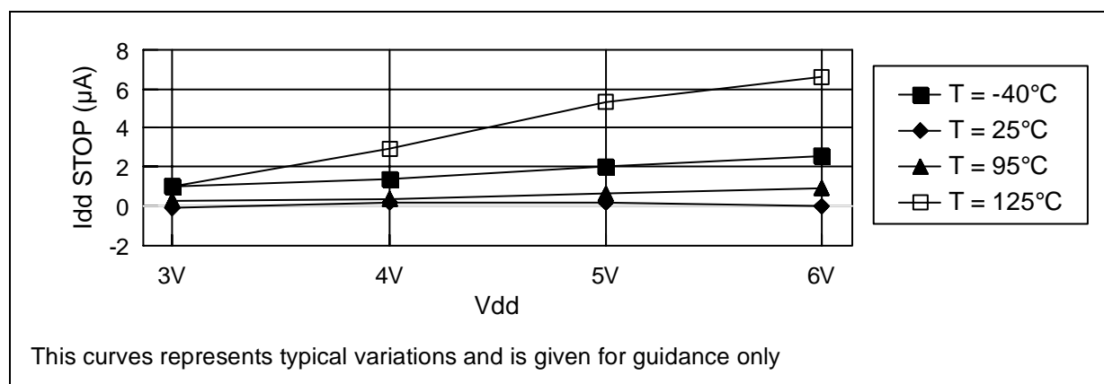
Figure 39. Idd STOP versus V_{DD} for ROM devices
