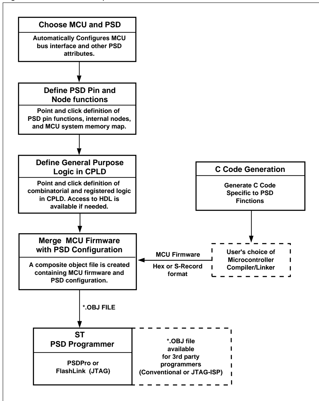
Figure 2. PSDsoft Development Tool
