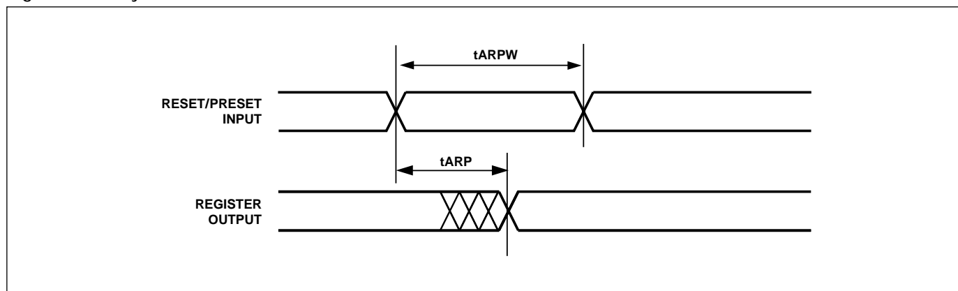
Figure 42. Asynchronous Reset/Preset
