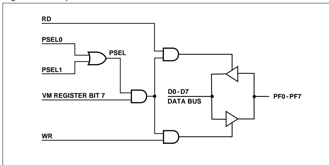
Figure 25. Peripheral I/O Mode
