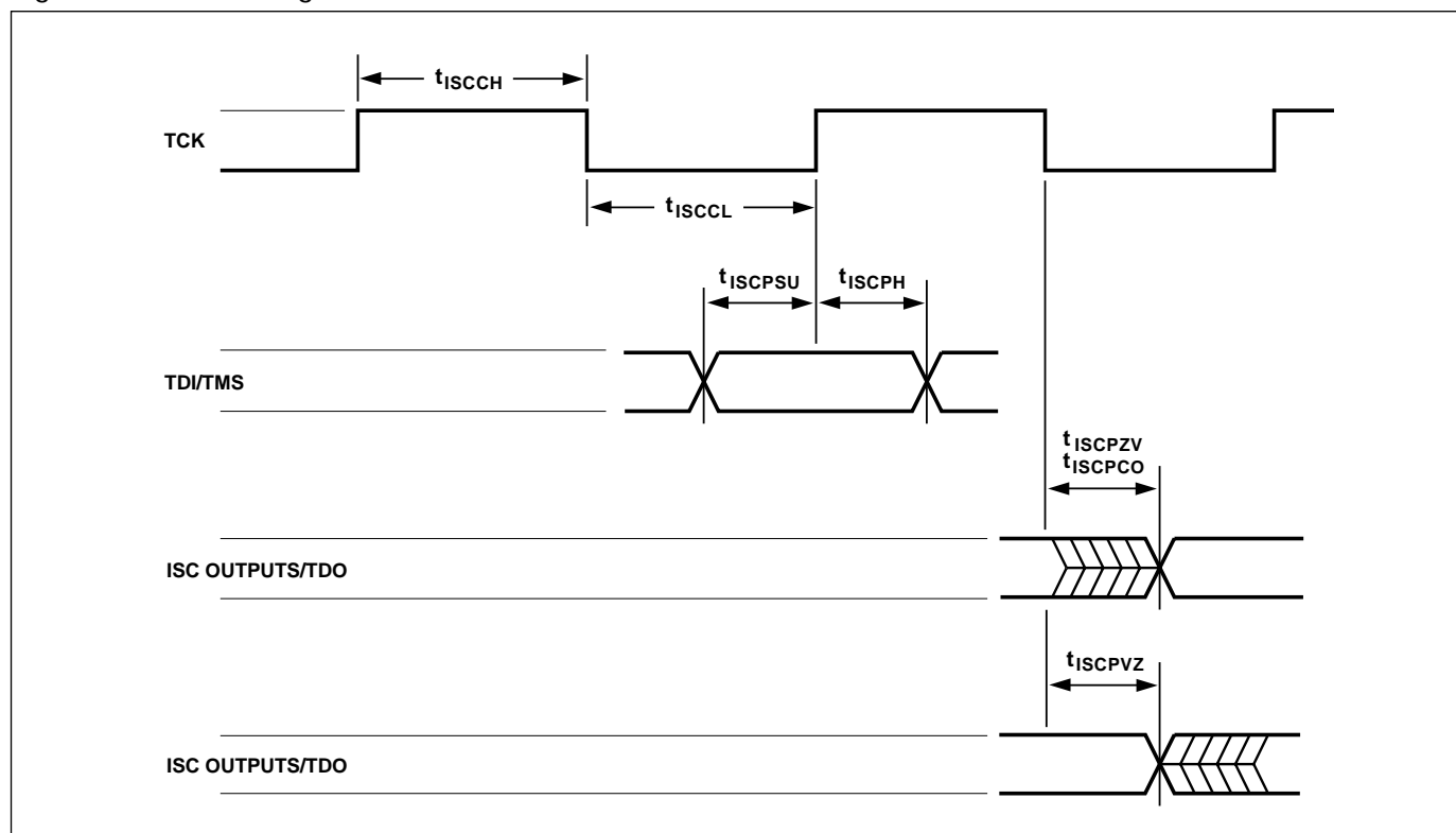
Figure 43. ISC Timing
