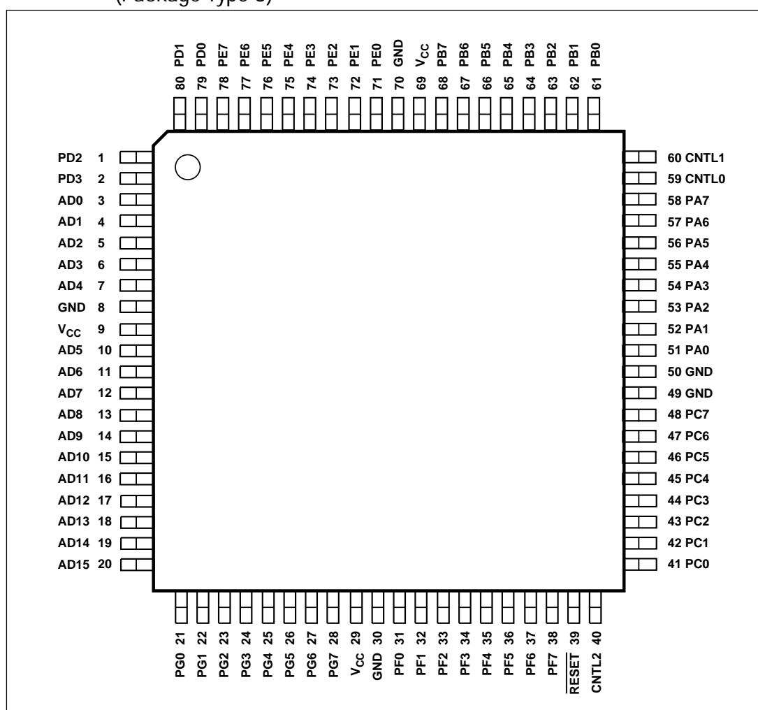
Figure 48. Drawing U5 – 80-Pin Plastic Thin Quad Flatpack (TQFP) (Package Type U)
