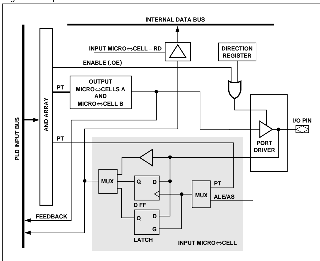
Figure 14. Input Micro \leftrightarrow Cell
