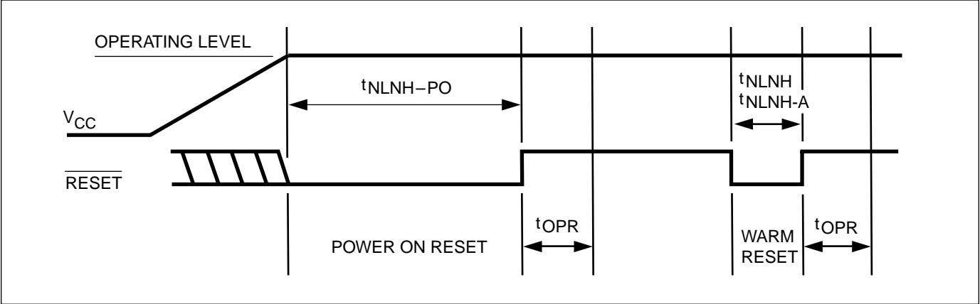
Figure 44. Reset Timing
