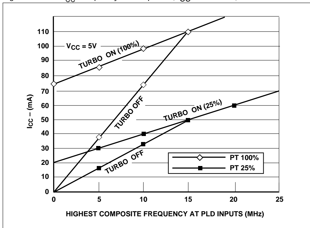
Figure 32. PLD I_{CC} /FrequencyConsumption ( V_{CC} = 5\text{ V} \pm 10\% )
