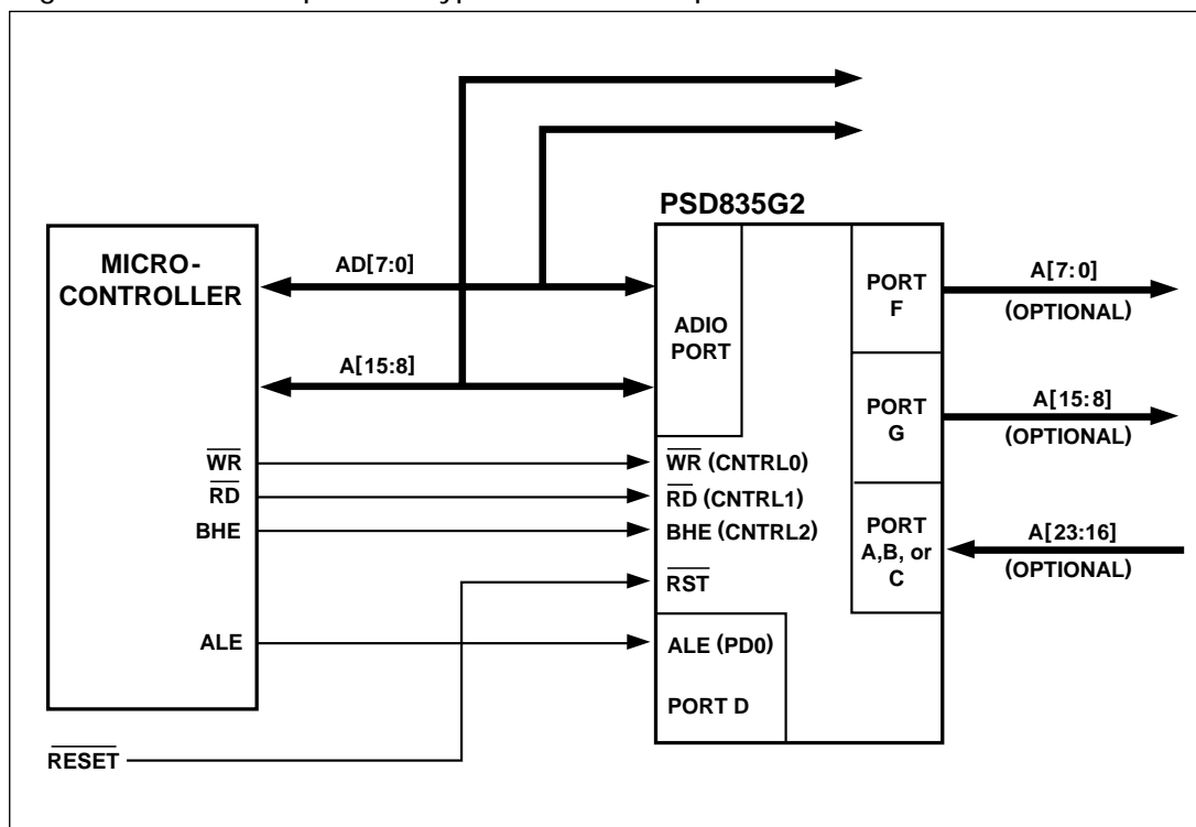
Figure 17. An Example of a Typical 8-Bit Multiplexed Bus Interface
