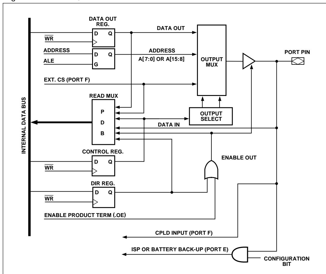
Figure 28. Ports E, F and G Structure
