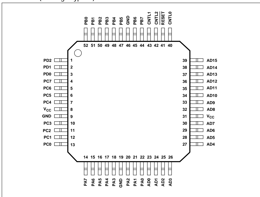
Figure 50. Drawing M3 – 52-Pin Plastic Quad Flatpack (PQFP) (Package Type M)
