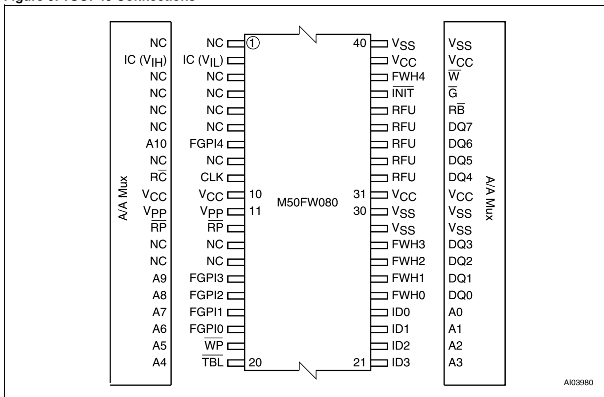
Figure 6. TSOP40 Connections
