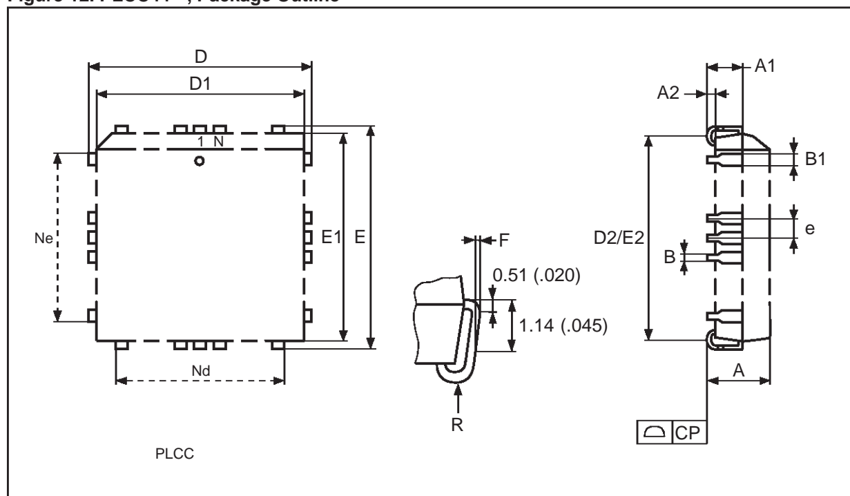
Figure 12. PLCC44 - , Package Outline
