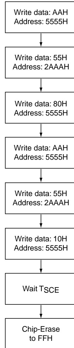
FIGURE 19: SOFTWARE CHIP-ERASE COMMAND CODES
