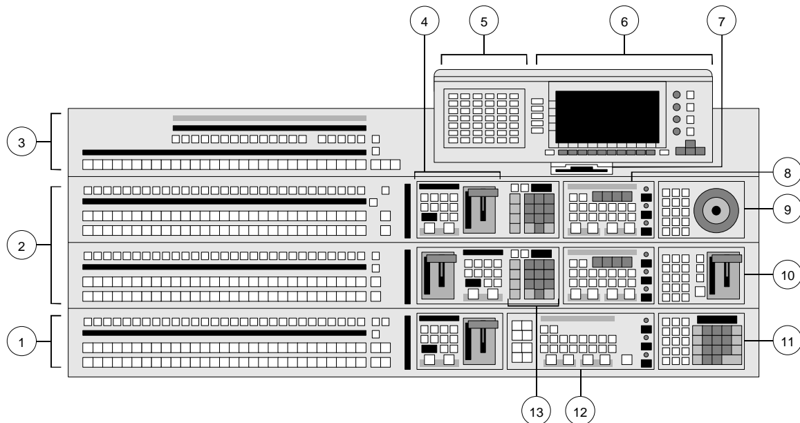
DVS-7250 Control Panel (Euro Style) Top View
