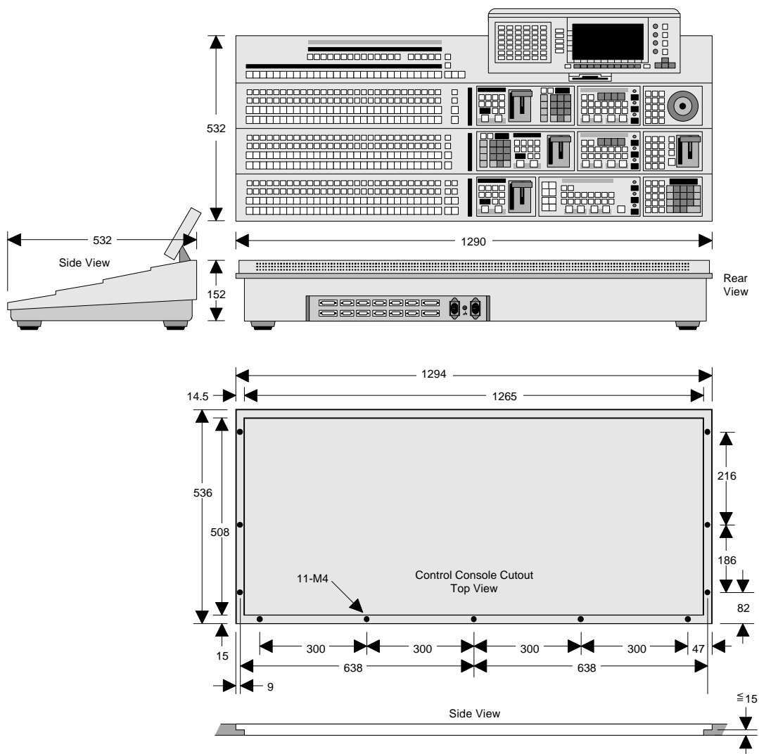
DVS-7250 External Control Panel Dimensions
