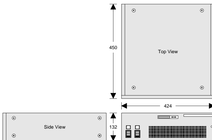
BKDS-7700 External Chassis Dimensions
