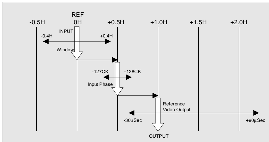
DVS-7250 System Phase Timing Chart
