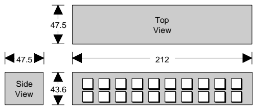
BKDS-8061 External Shot Box Control Unit Dimensions
