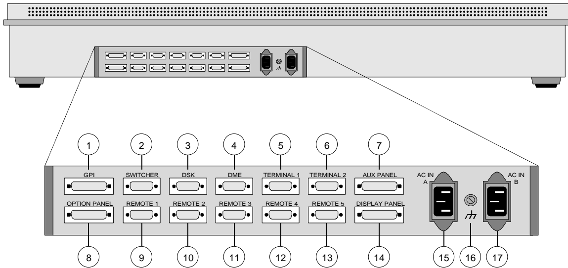
DVS-7250 Control Panel Rear View
