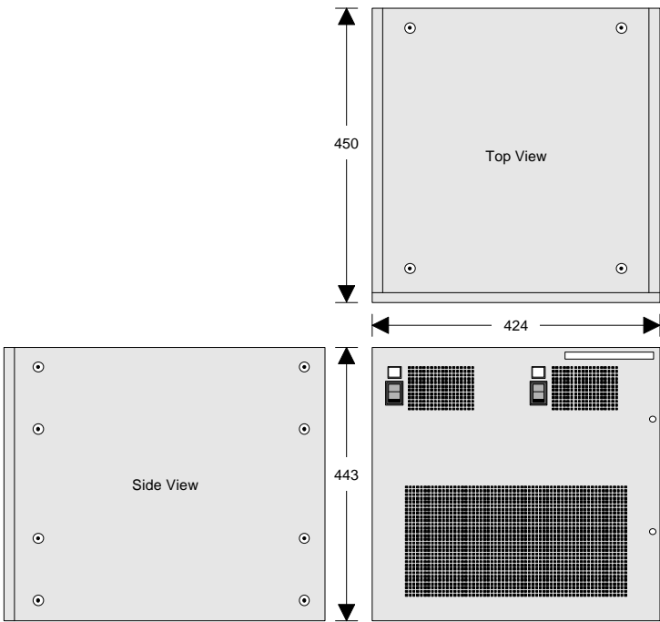
DVS-7250 External Chassis Dimensions
