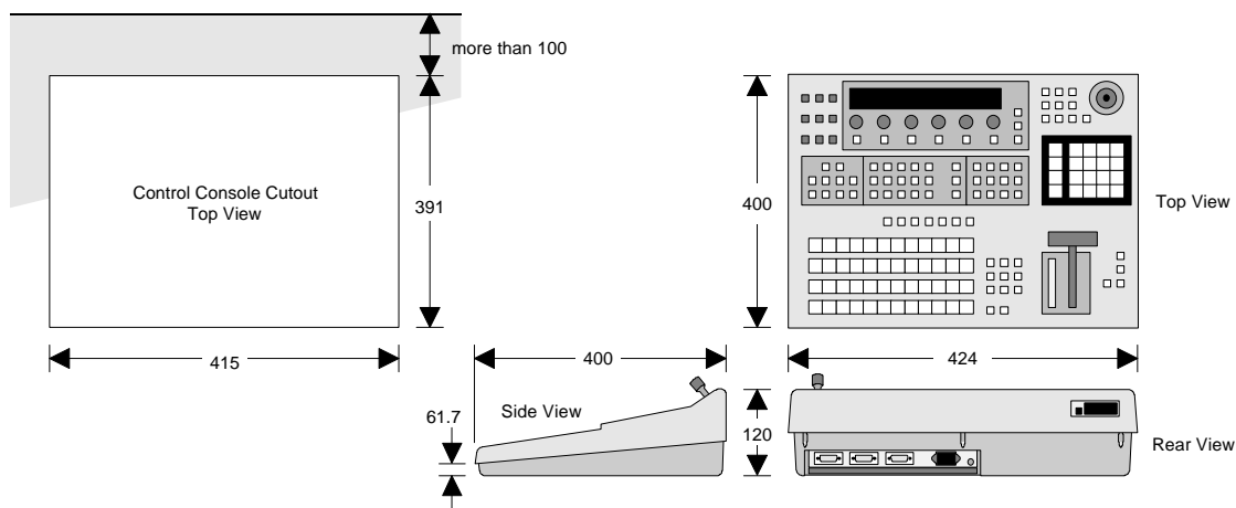
BKDS-2010 External Control Panel Dimensions
