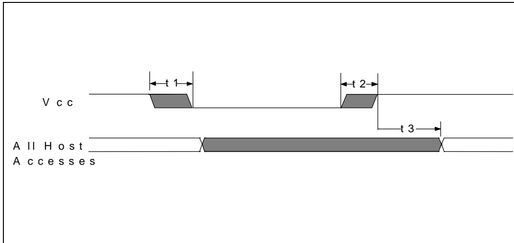
FIGURE 3 - POWER-UP TIMING
