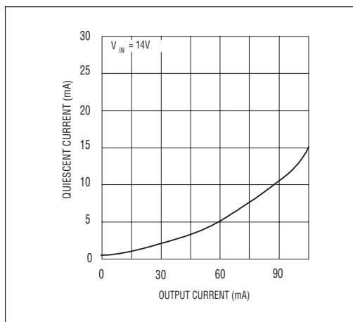
Figure 2. Quiescent Current
