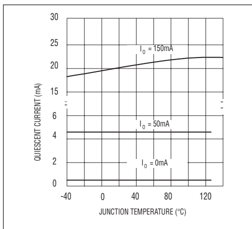
Figure 1. Quiescent Current
