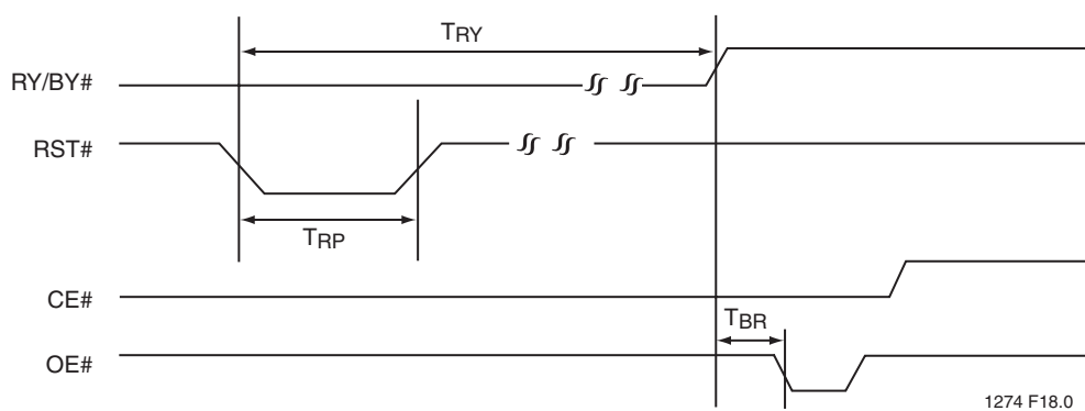
FIGURE 20: RST# TIMING DIAGRAM (DURING SECTOR- OR BLOCK-ERASE OPERATION)
