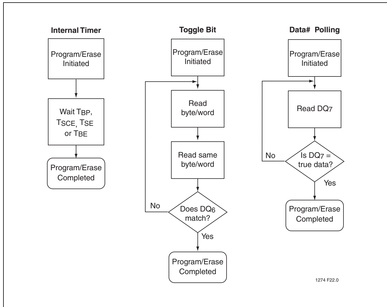
FIGURE 24: WAIT OPTIONS
