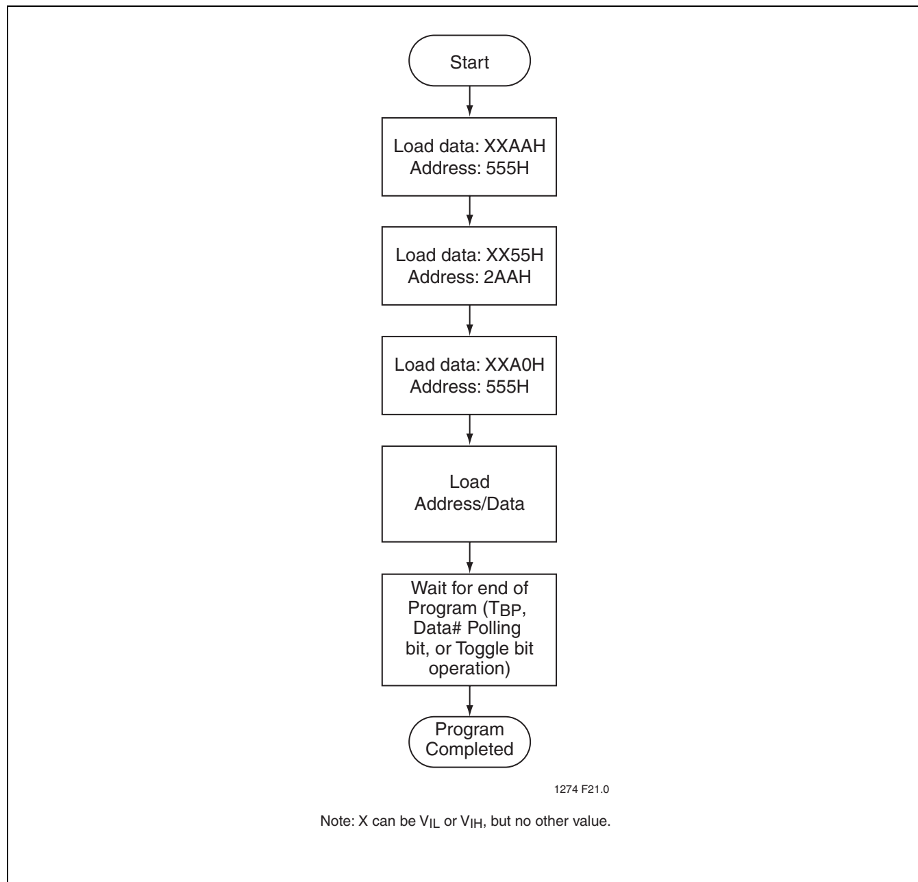
FIGURE 23: PROGRAM ALGORITHM
