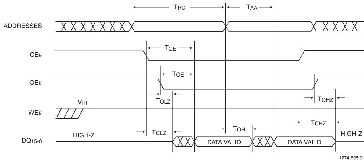
FIGURE 7: READ CYCLE TIMING DIAGRAM
