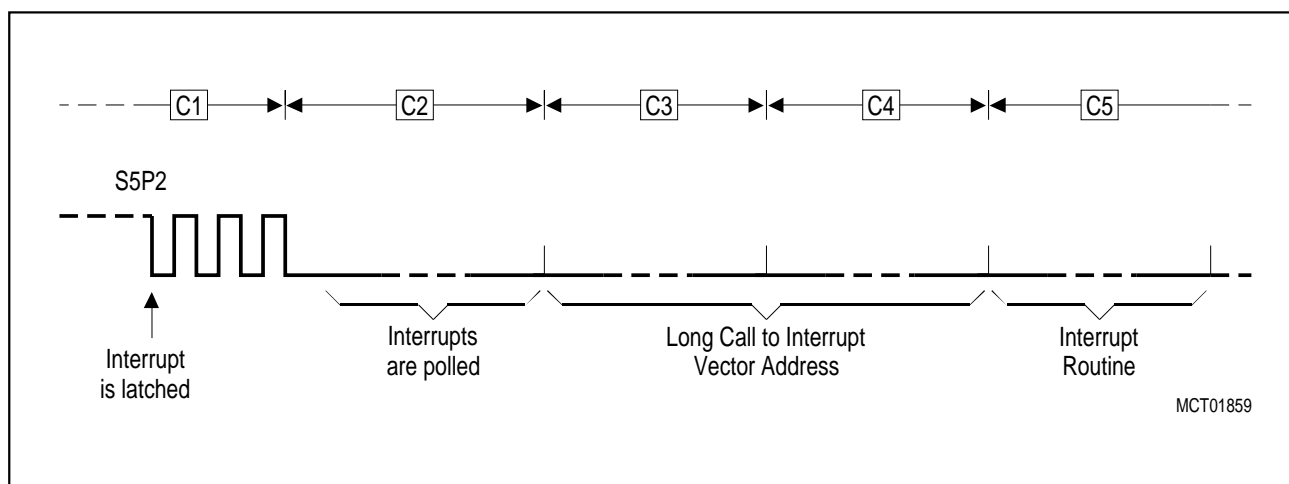
Figure 2-5 Interrupt Detection/Entry Diagram
