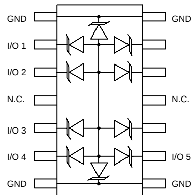
Connection Diagram
