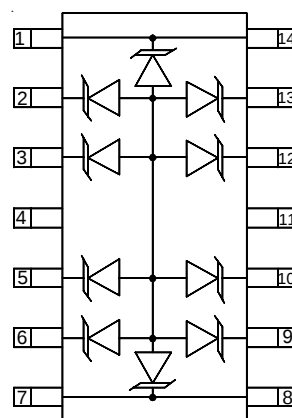
SO-14 (Top View)
