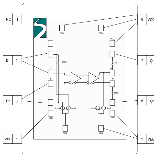
SK10/100EL16TD Input Termination with 100Ω Resistor Across the Differential Inputs and 8 mA Output Source Termination with 50Ω Series Resistor
