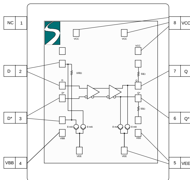
SK10/100EL16TC Input Termination with 100Ω Resistor Across the Differential Inputs and 8 mA Output Source Termination
