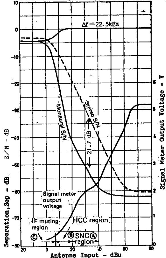
SNC Characteristic (Fig 3b)
