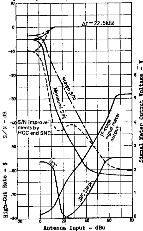
SNC Characteristic (Fig 3a)
