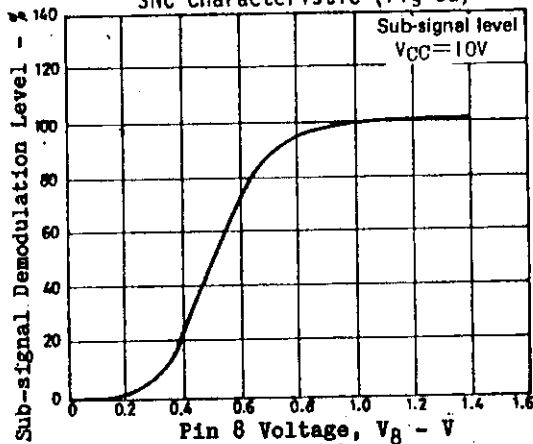
SNC Characteristic (Fig 3a)
