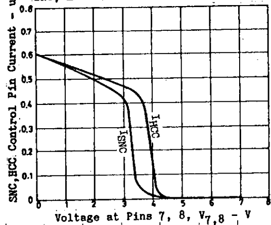
SNC, HCC Control Pin Current (Fig.6)
