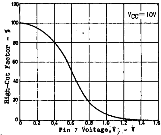
HCC Characteristic (Fig 8)
