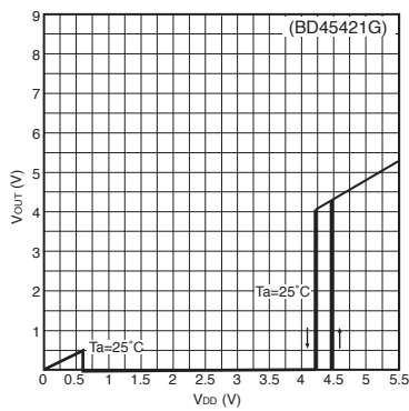
I/O characteristic
