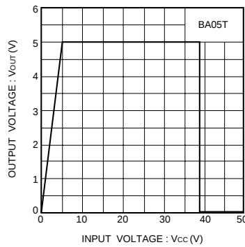
Fig. 10 Over voltage protection characteristics
