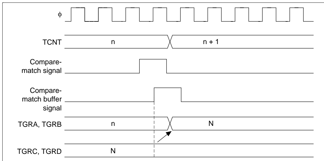
Figure 12.67 Buffer Operation Timing (Compare-Match)
