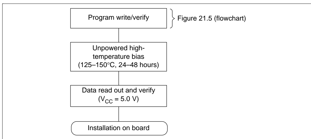
Figure 21.8 Screening Flow
