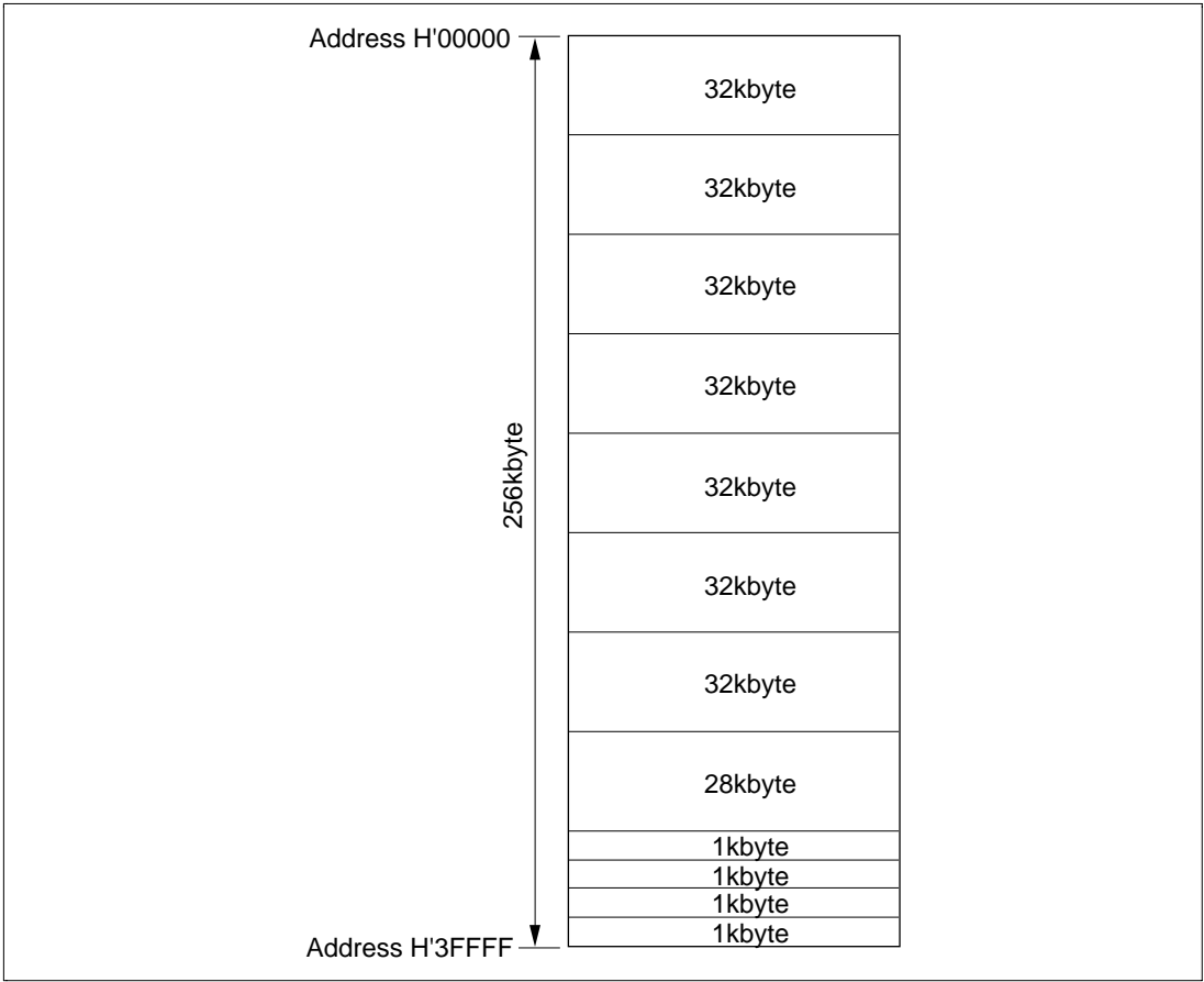
Figure 22.7 Block Configuration
