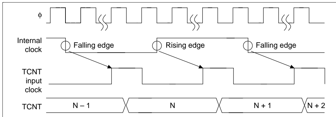
Figure 12.59 TCNT Count Timing during Internal Clock Operation
