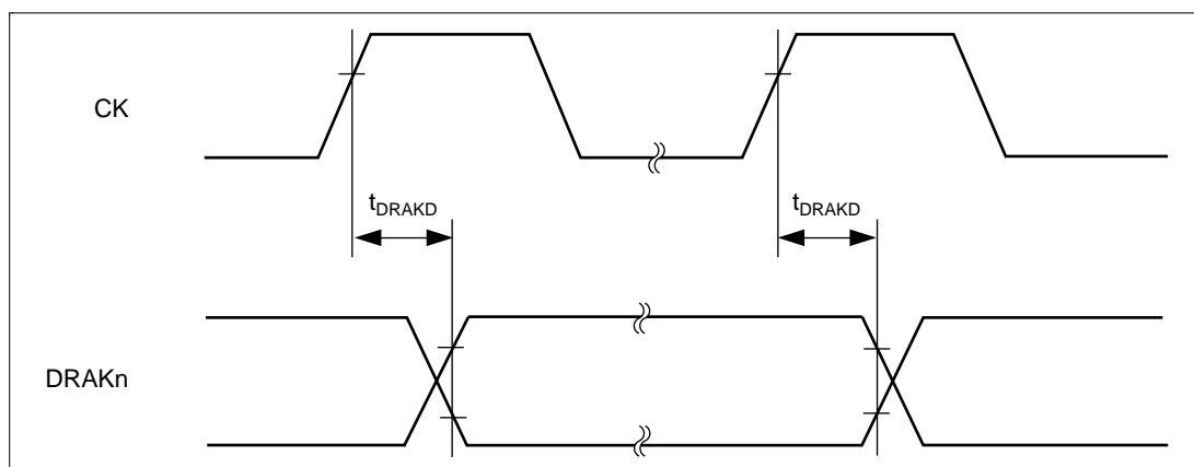
Figure 25.22 DRAKn Output Delay Time
