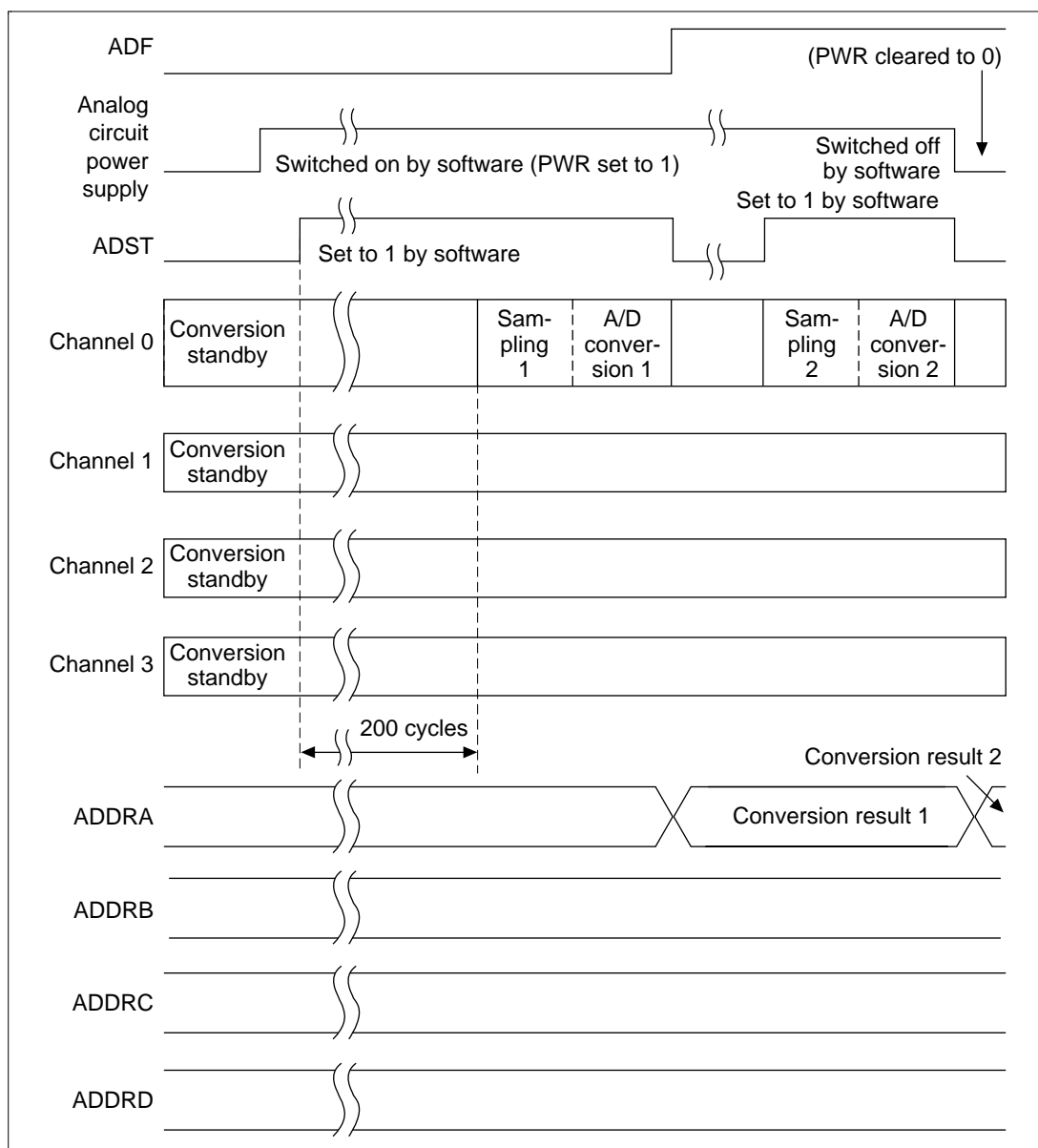
Figure 15.11 Conversion Start Operation (High-Speed Start Mode)
