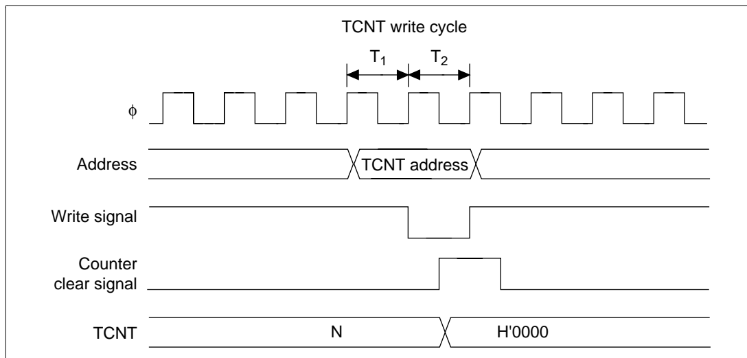
Figure 12.77 TCNT Write and Clear Contention
