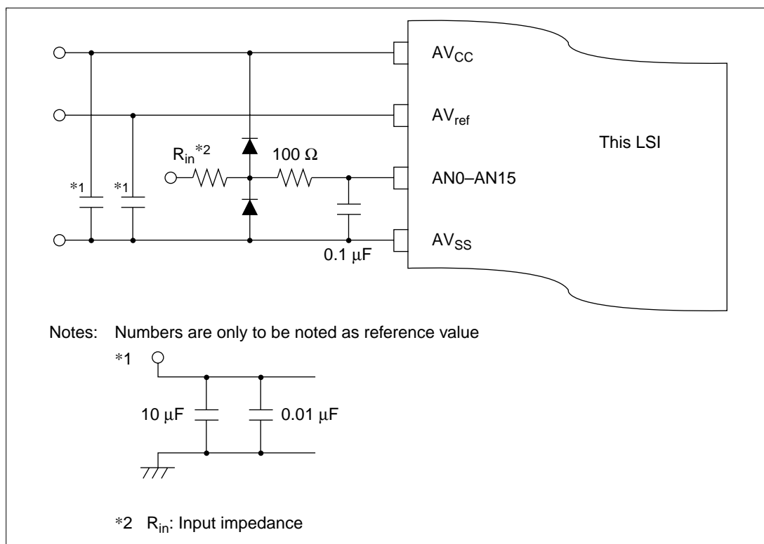
Figure 16.8 Example of Analog Input Pin Protection Circuit
