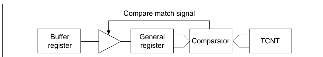
Figure 12.17 Compare Match Buffer Operation
