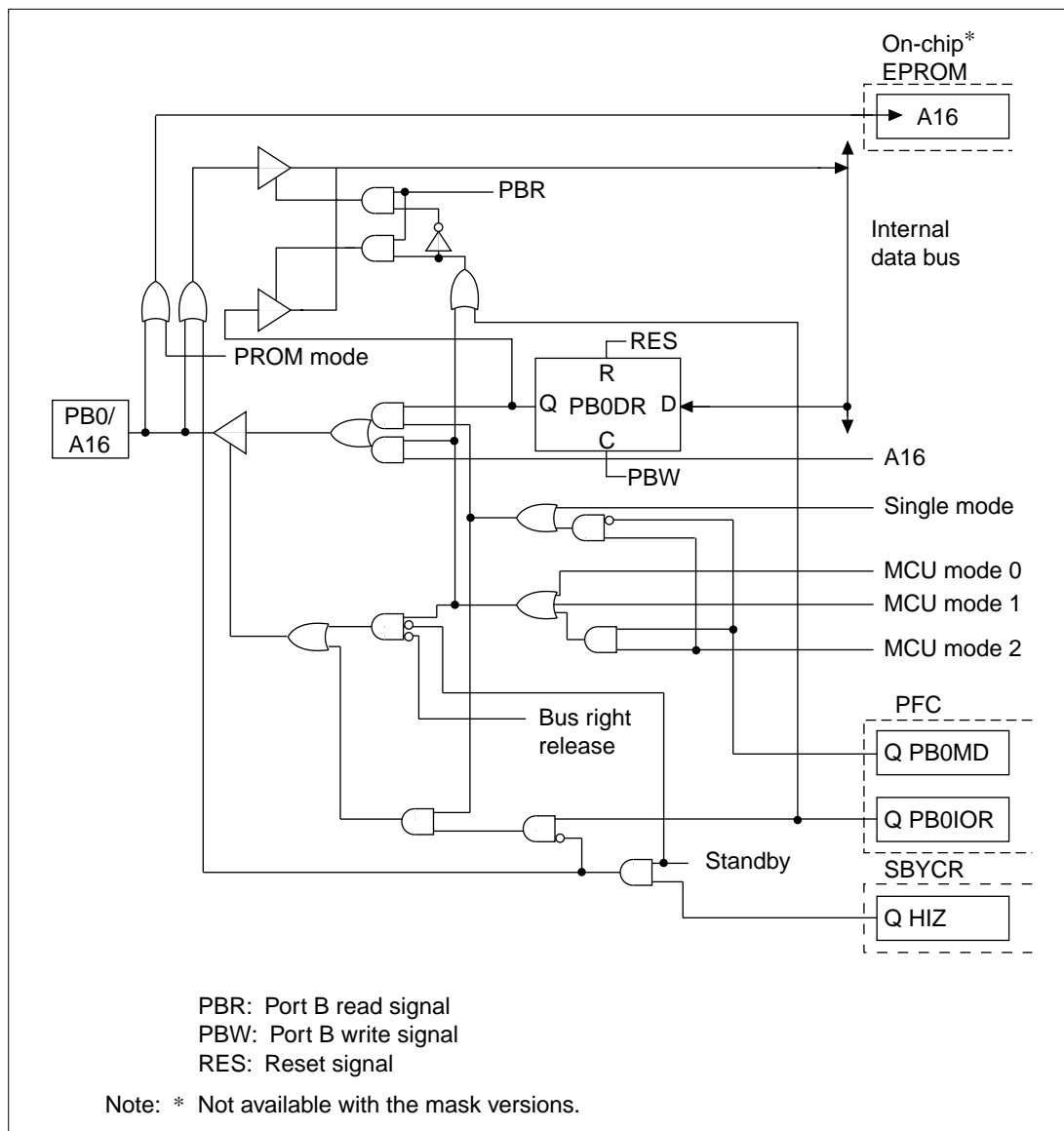
Figure B.14 PB0/A16 Block Diagram
