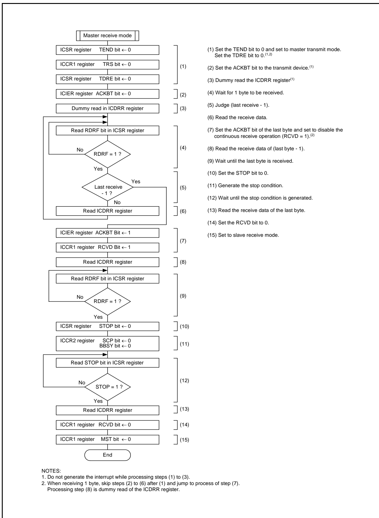
Figure 16.47 Example of Register Setting in Master Receive Mode (Clock Synchronous Serial Mode)
