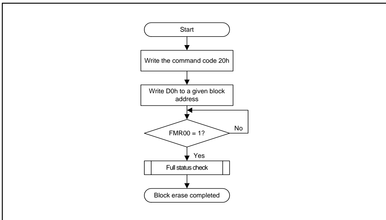
Figure 18.13 Block Erase Command (When Not Using Erase-Suspend Function)
