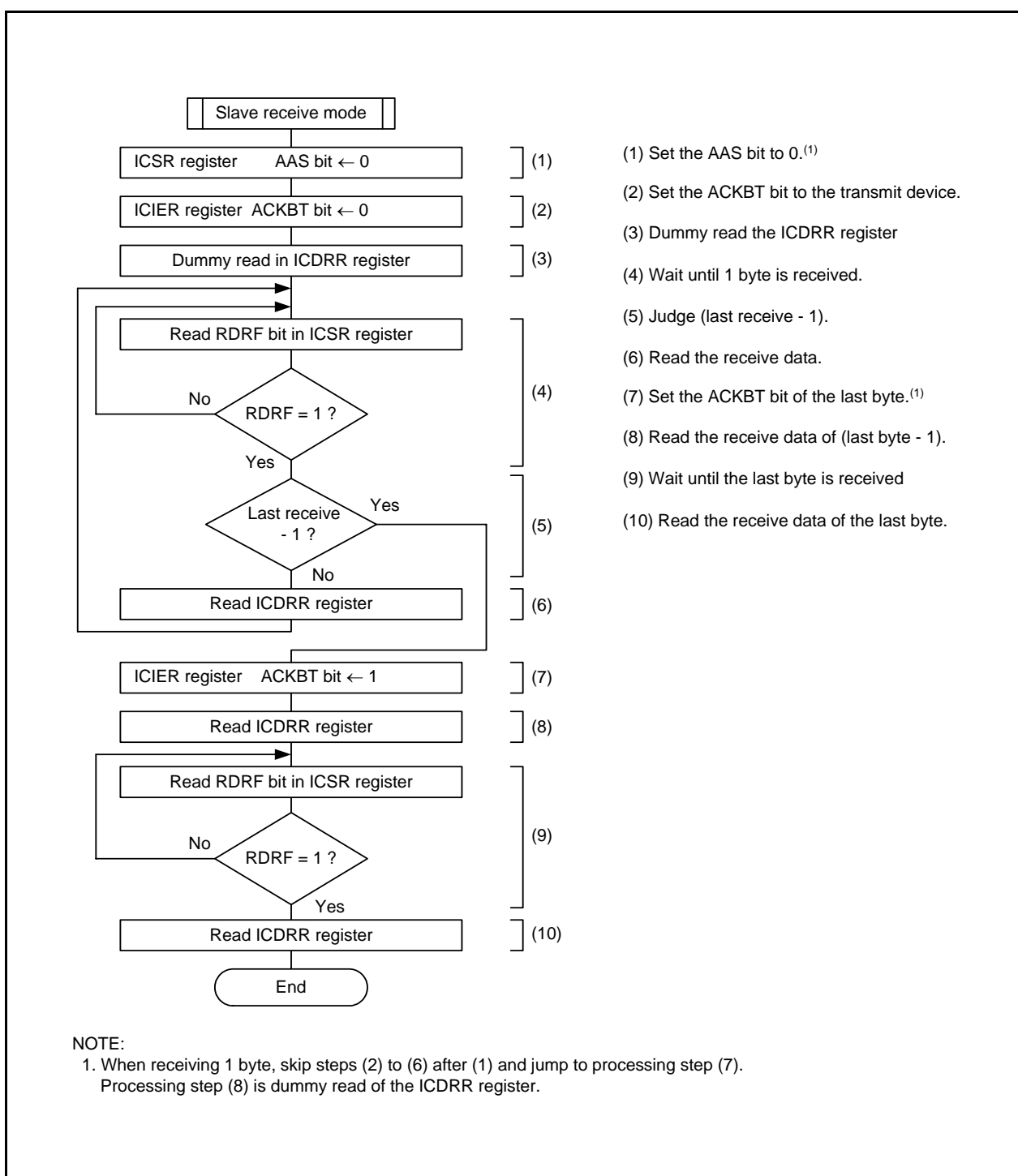
Figure 16.49 Example of Register Setting in Slave Receive Mode
