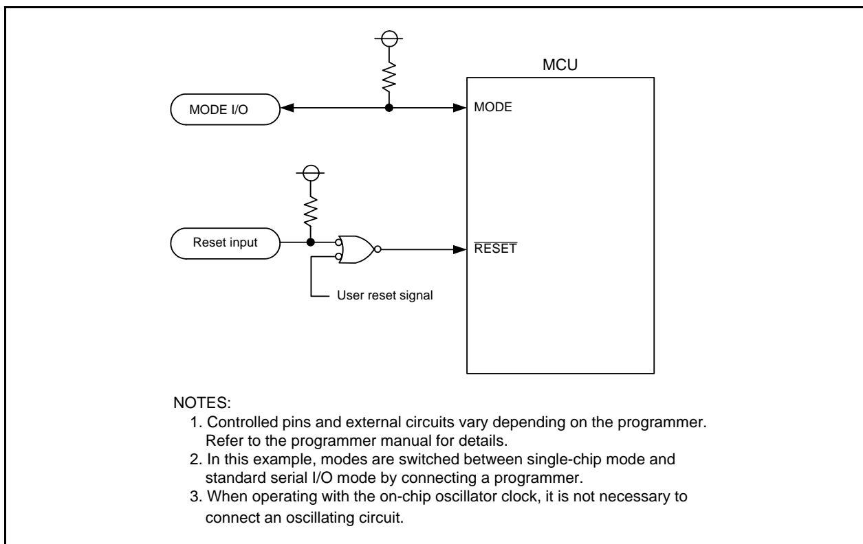
Figure 18.18 Pin Processing in Standard Serial I/O Mode 3
