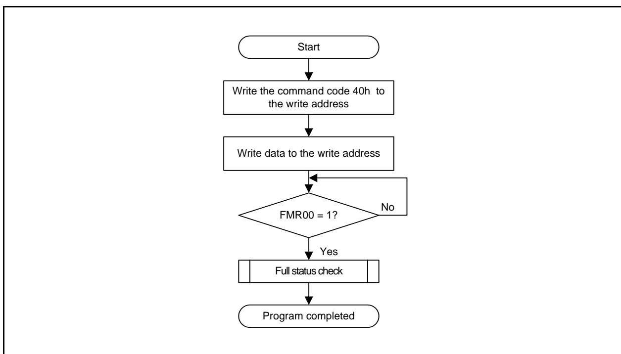
Figure 18.12 Program Command
