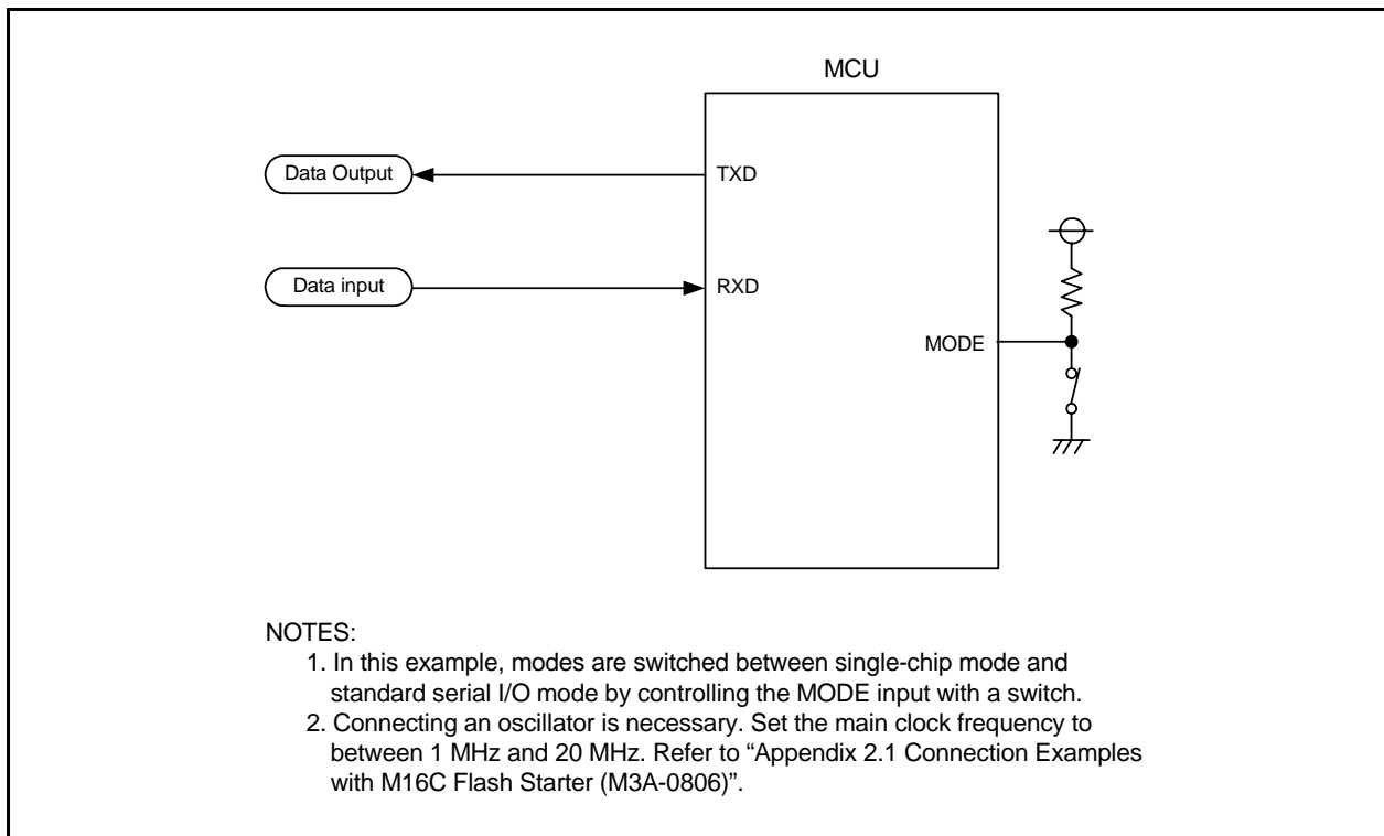
Figure 18.17 Pin Processing in Standard Serial I/O Mode 2
