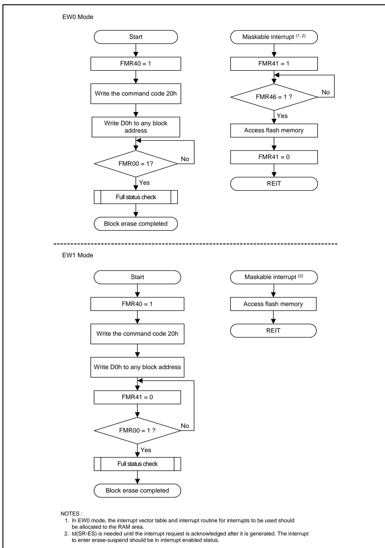
Figure 18.14 Block Erase Command (When Using Erase-Suspend Function)
