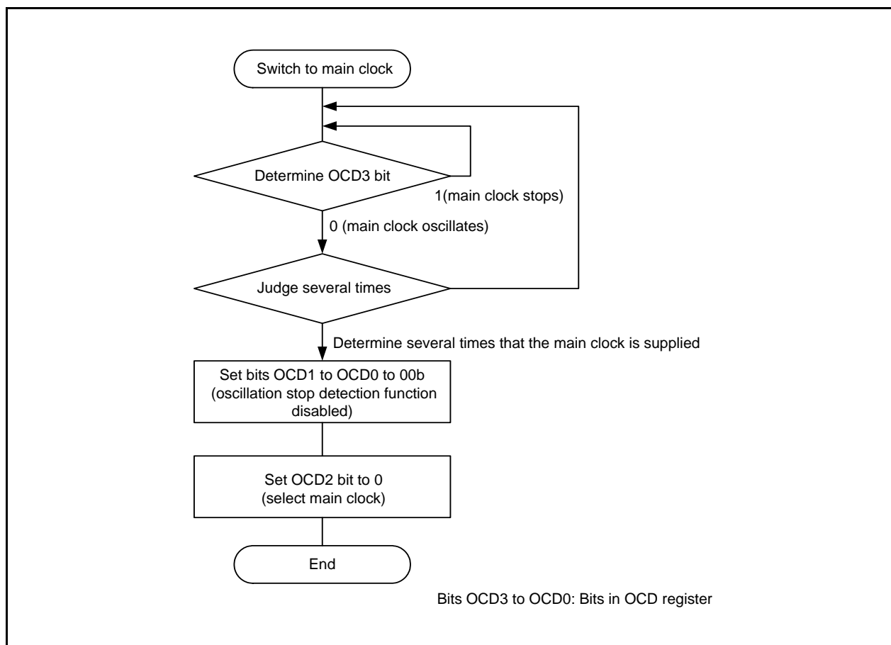
Figure 10.9 Procedure for Switching Clock Source from Low-Speed On-Chip Oscillator to Main Clock
