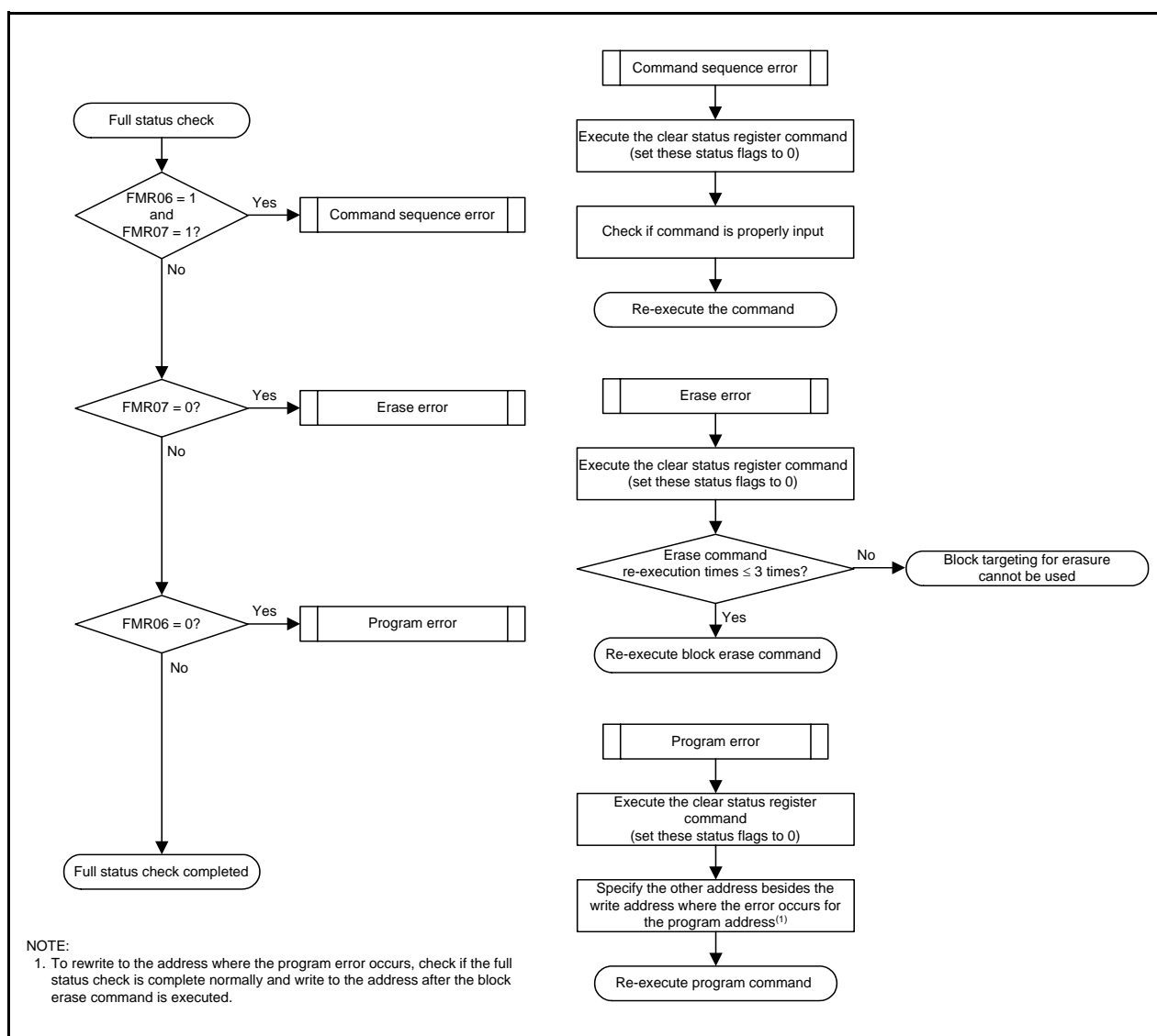
Figure 18.15 Full Status Check and Handling Procedure for Individual Errors
