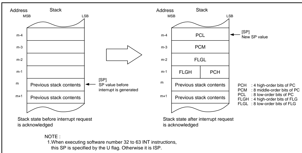
Figure 12.7 Stack State Before and After Acknowledgement of Interrupt Request
