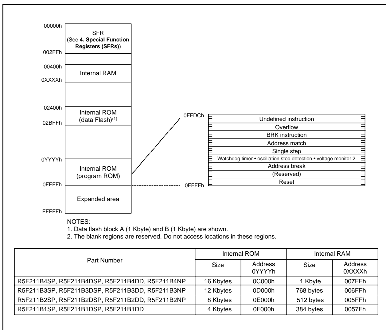
Figure 3.2 Memory Map of R8C/1B Group
