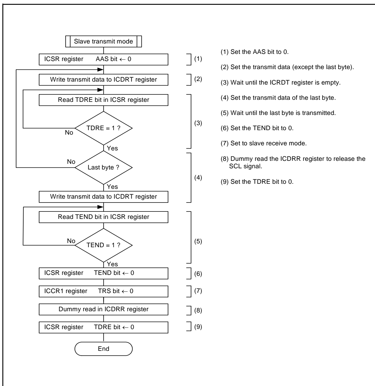
Figure 16.48 Example of Register Setting in Slave Transmit Mode (Clock Synchronous Serial Mode)
