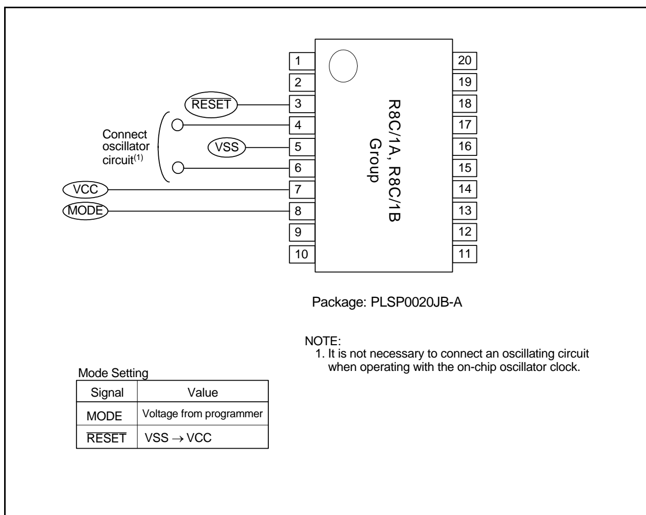
Figure 18.16 Pin Connections for Standard Serial I/O Mode 3
