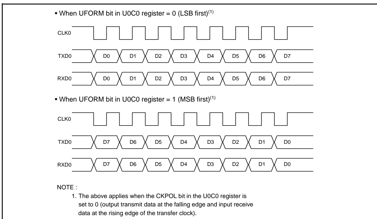
Figure 15.9 Transfer Format
