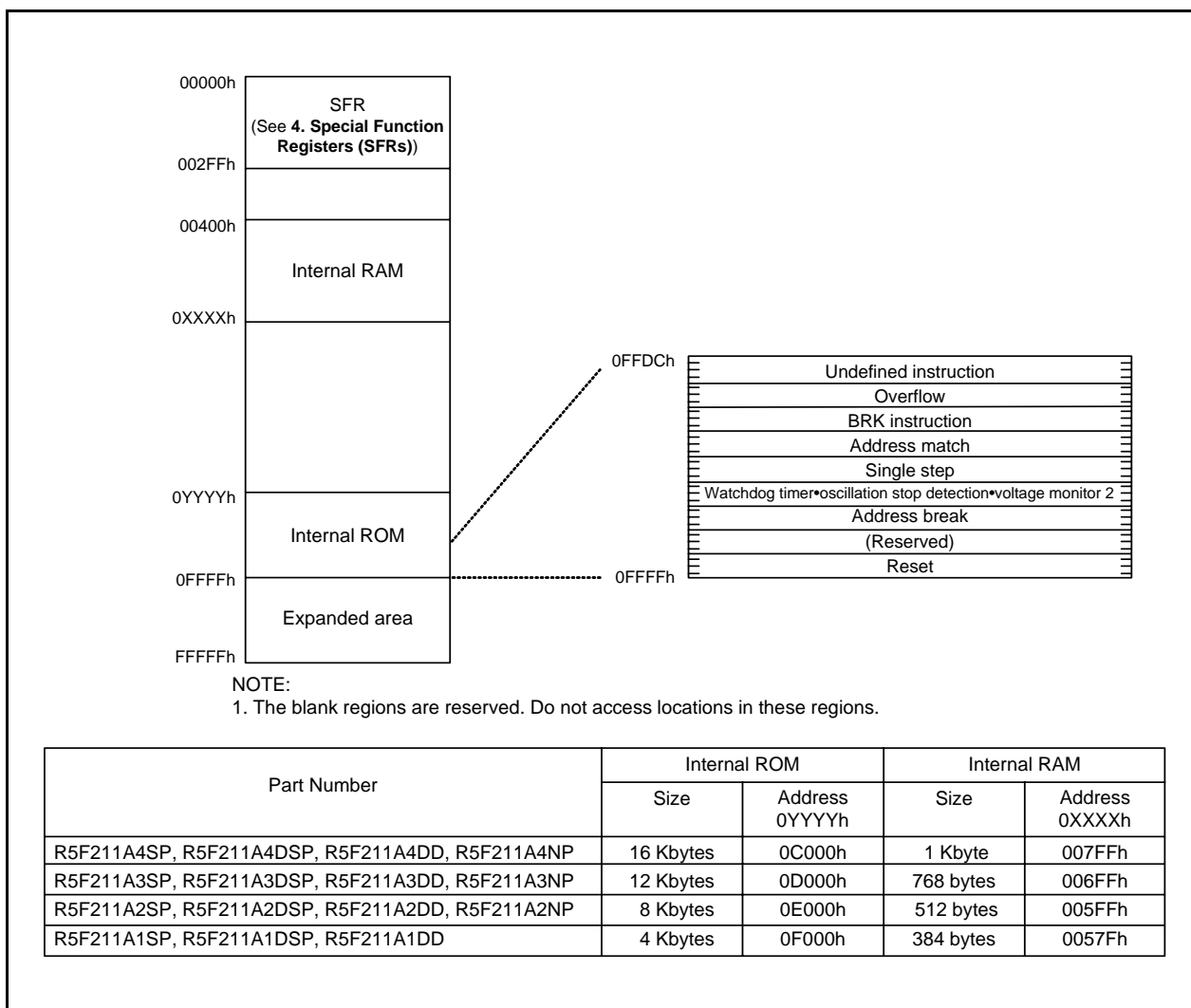
Figure 3.1 Memory Map of R8C/1A Group
