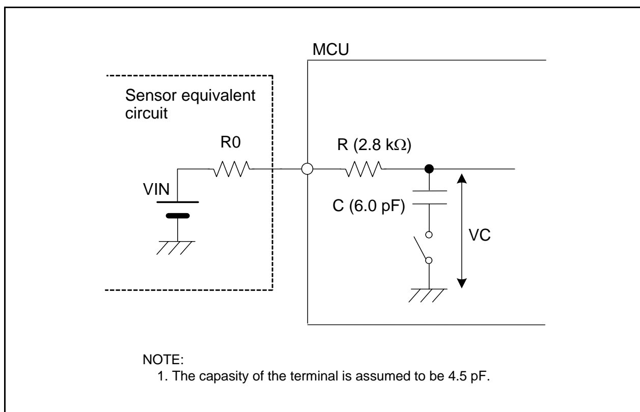
Figure 17.11 Analog Input Pin and External Sensor Equivalent Circuit
