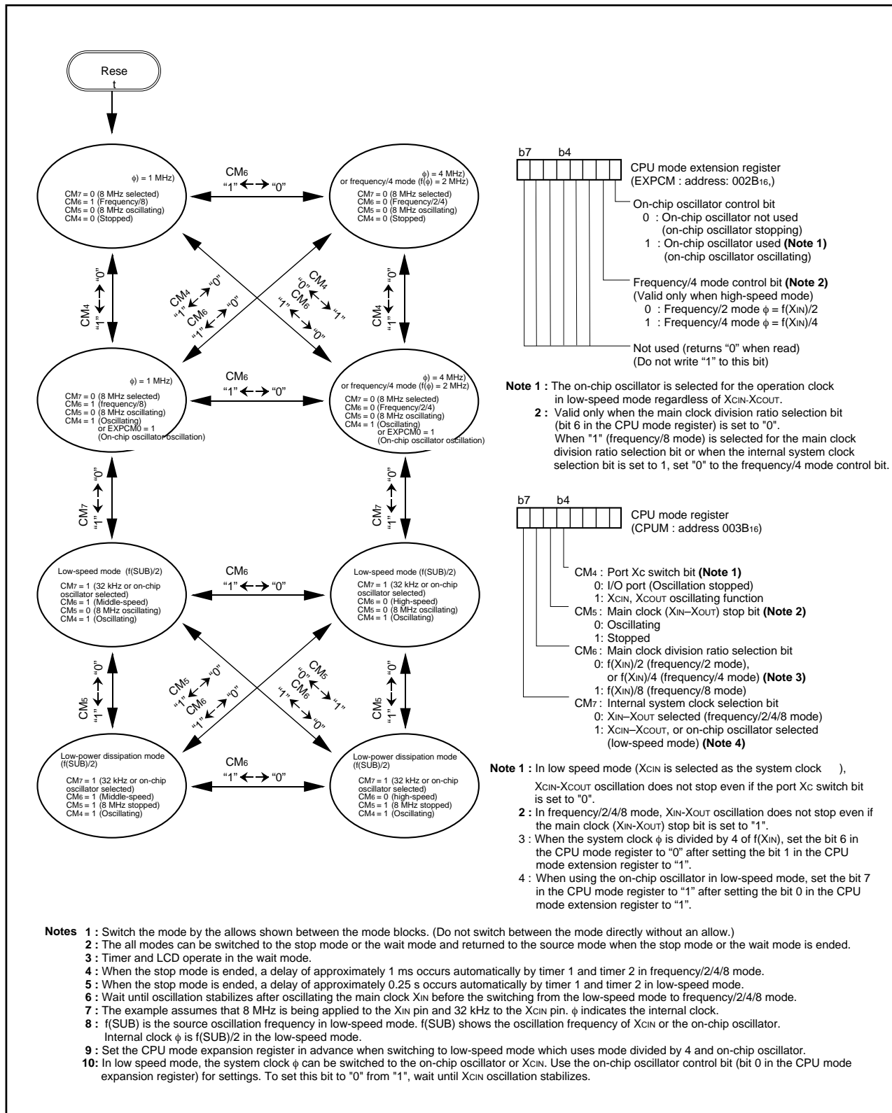
Fig. 57 State transitions of system clock
