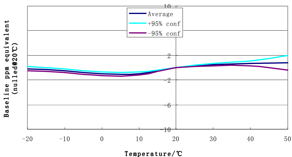
Baseline drift of 7R H 2 S sensor
