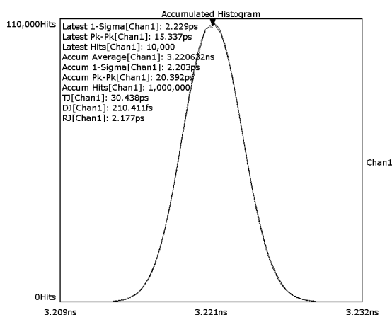
Figure 3: Period Jitter Histogram at 311.04 MHz
