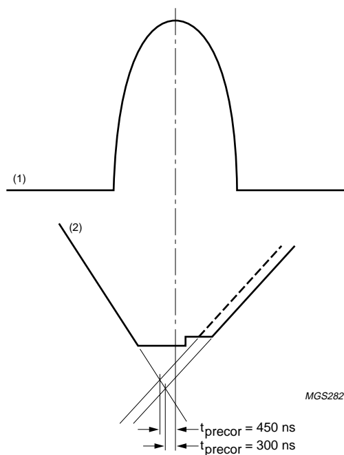
Fig.28 Definition of H-focus pre-correction.
