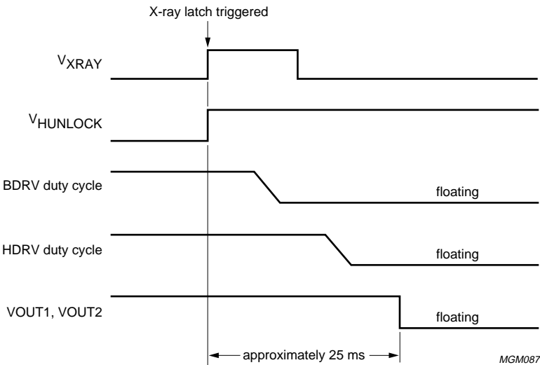
Fig.24 Activation of soft-down sequence via pin XRAY.
