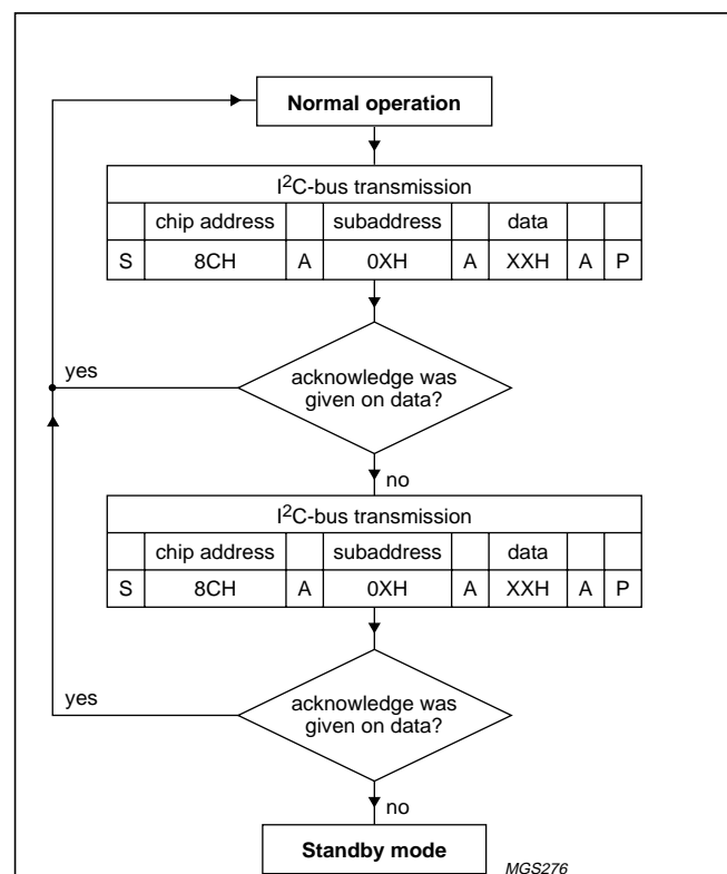
Fig.21 Possible standby mode detection.
