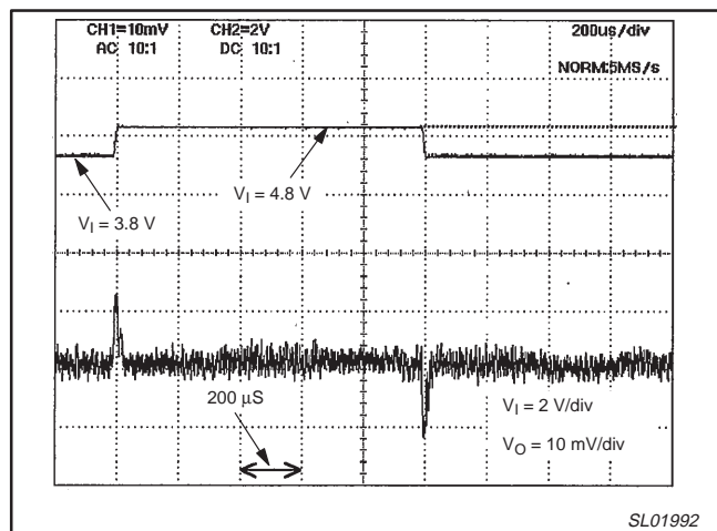
Figure 13. Line transient response.
