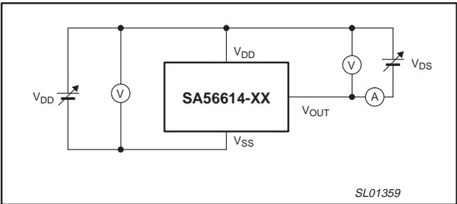
Figure 18. Test Circuit 3
