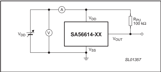
Figure 16. Test Circuit 1
