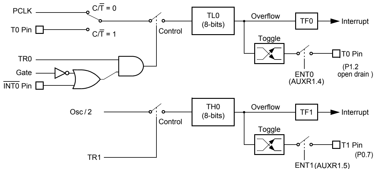
Figure 7-7: Timer/Counter 0 Mode 3 (two 8-bit counters)
