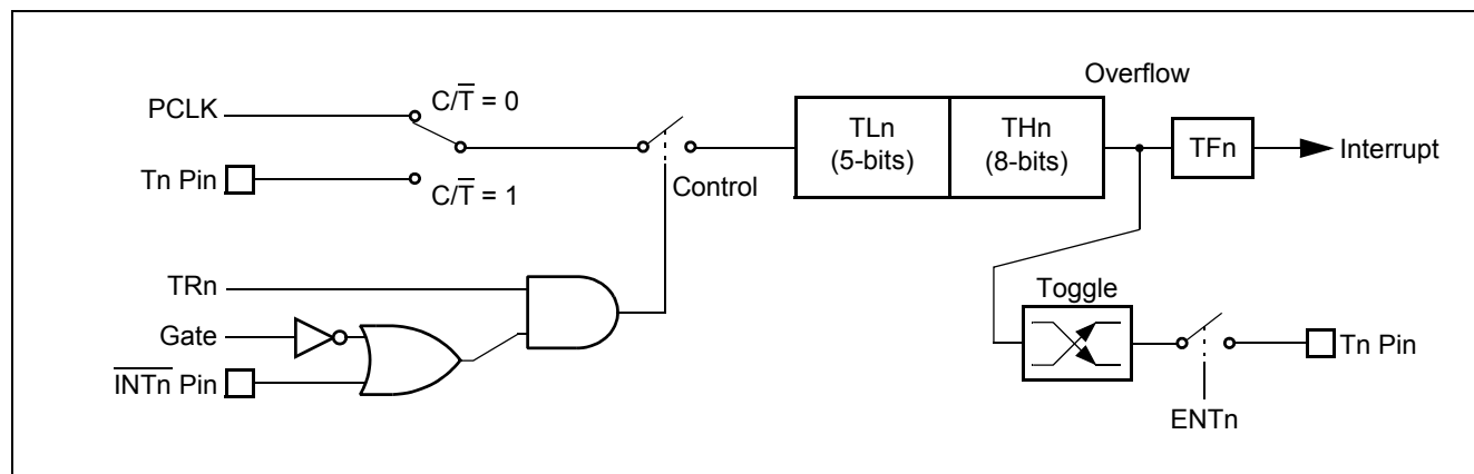
Figure 7-4: Timer/Counter 0 or 1 in Mode 0 (13-bit counter)
