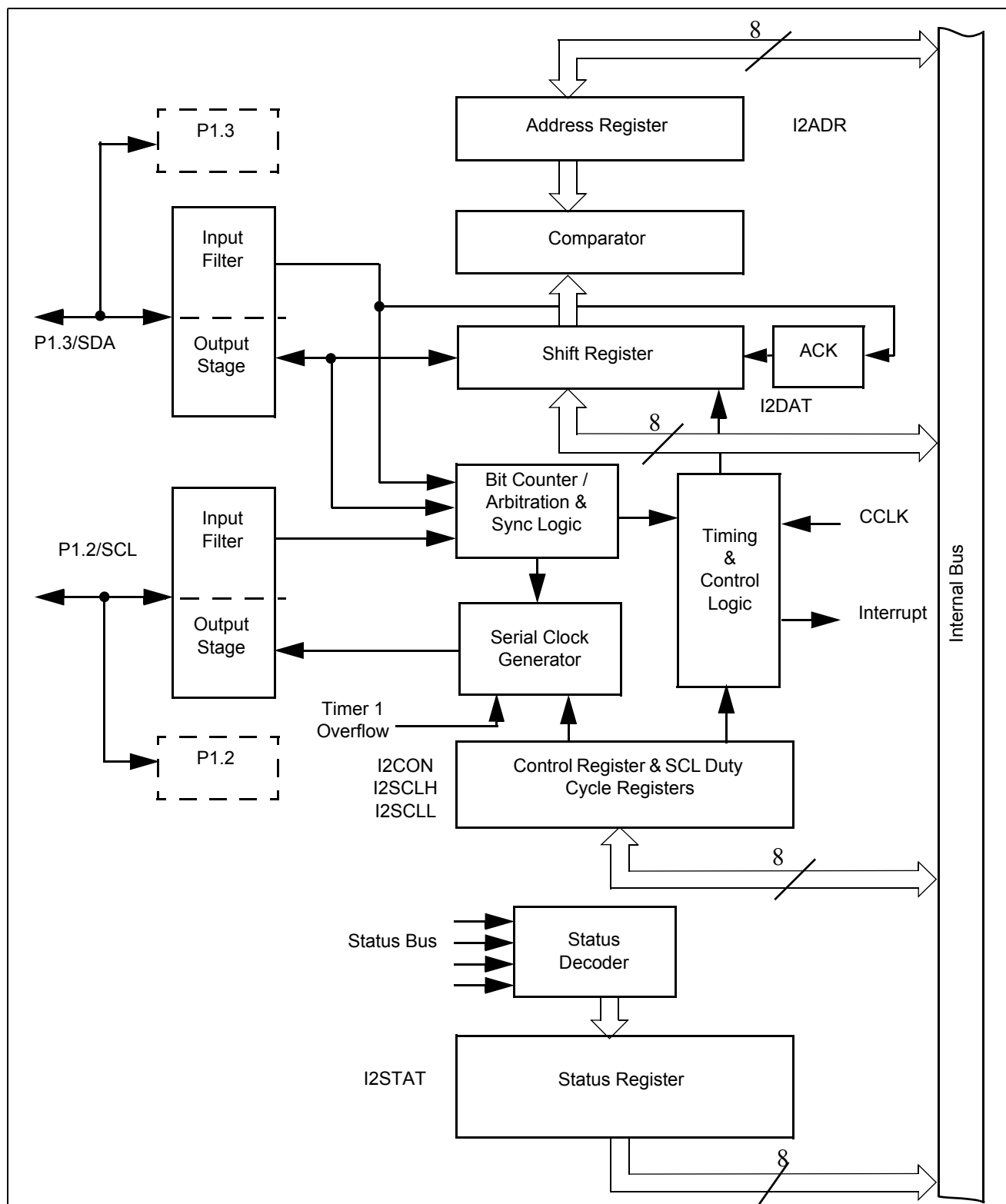
Figure 13: I 2 C-bus serial interface block diagram
