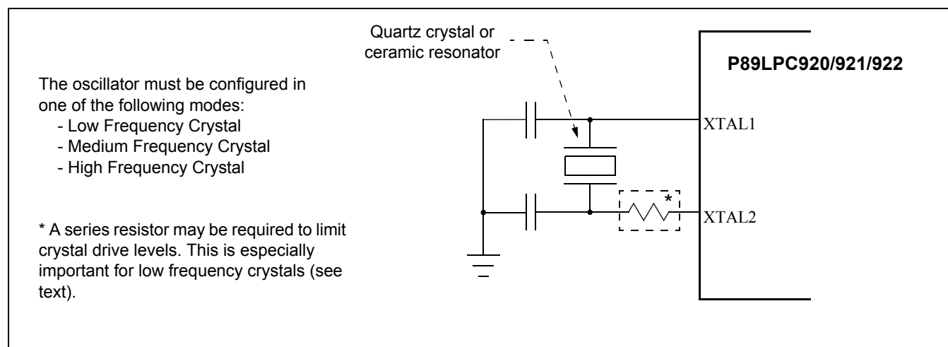
Figure 2-1: Using the crystal oscillator
