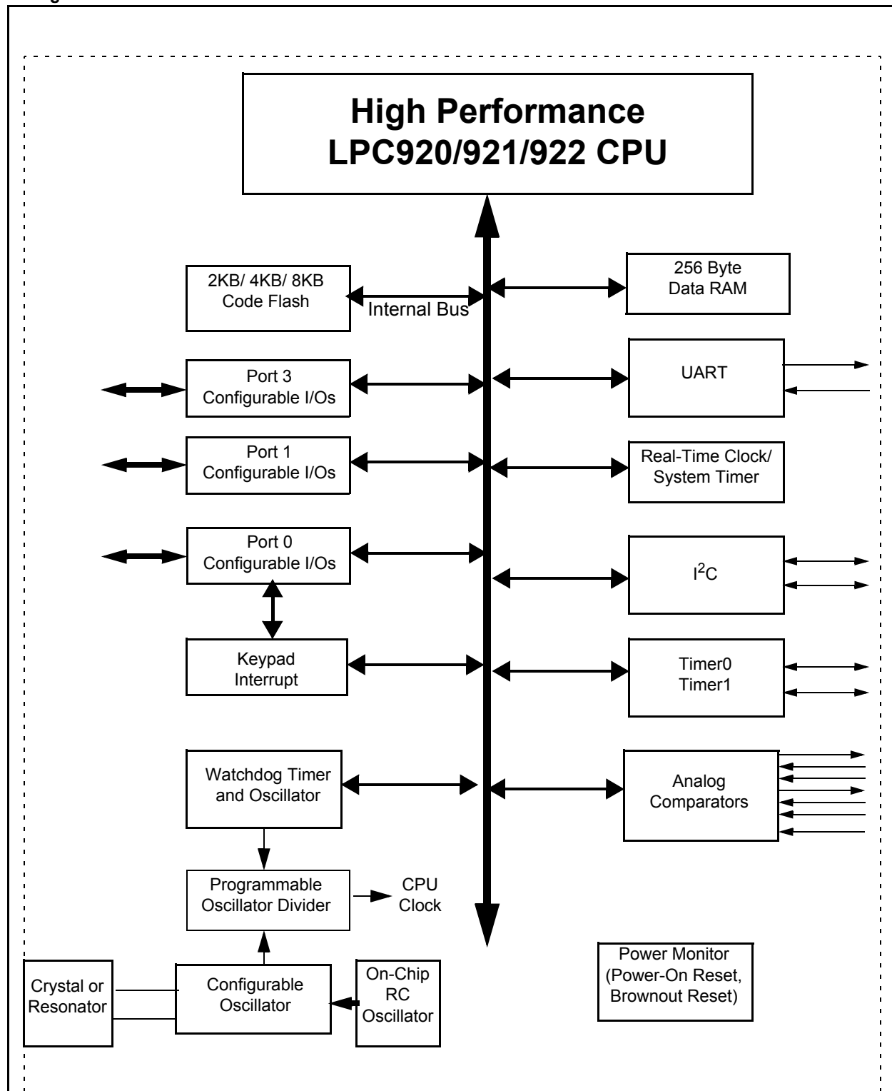
Block diagram
