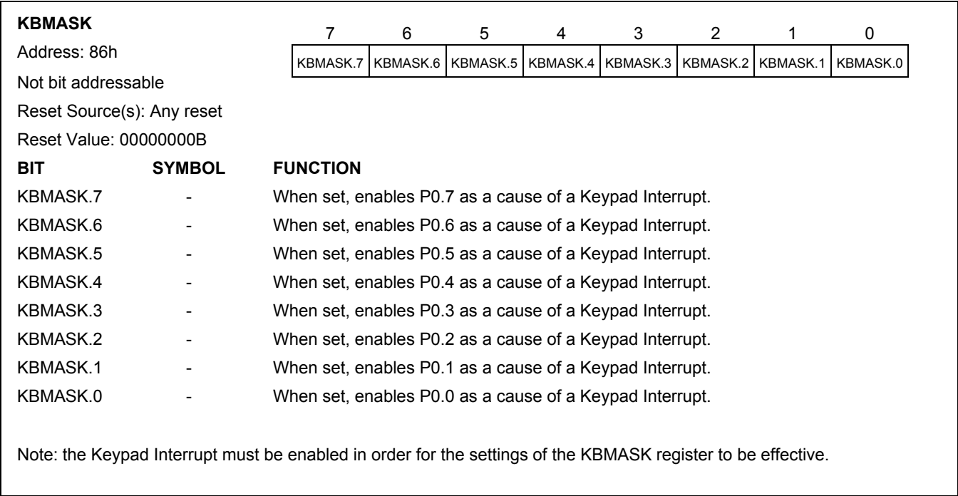
Figure 12-3: Keypad Interrupt Mask register (KBM)
