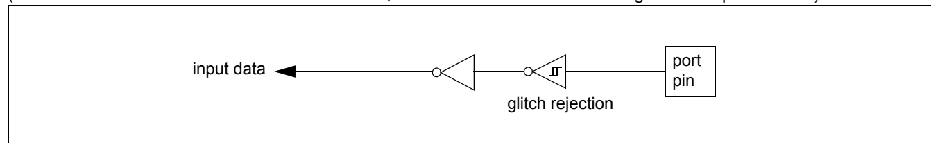
Figure 4-3: Input -only
