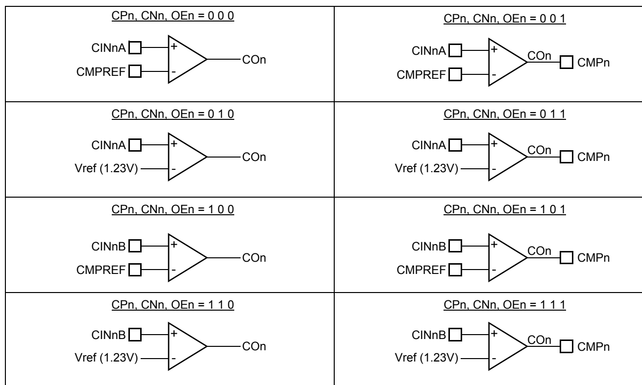
Figure 11-3: Comparator configurations
