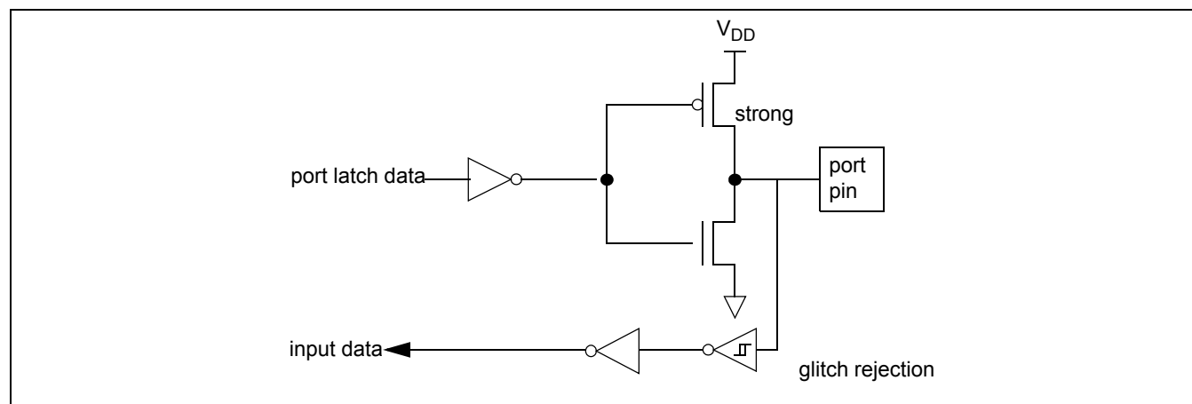
Figure 4-4: Push-pull output
