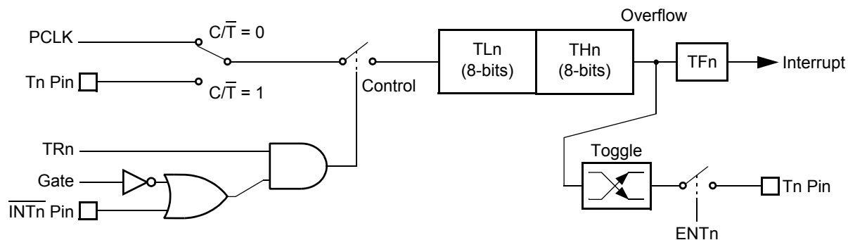
Figure 7-5: Timer/Counter 0 or 1 in Mode 1 (16-bit counter)
