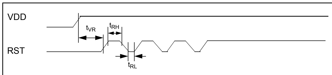
Figure 15-4: Forcing ISP Mode
