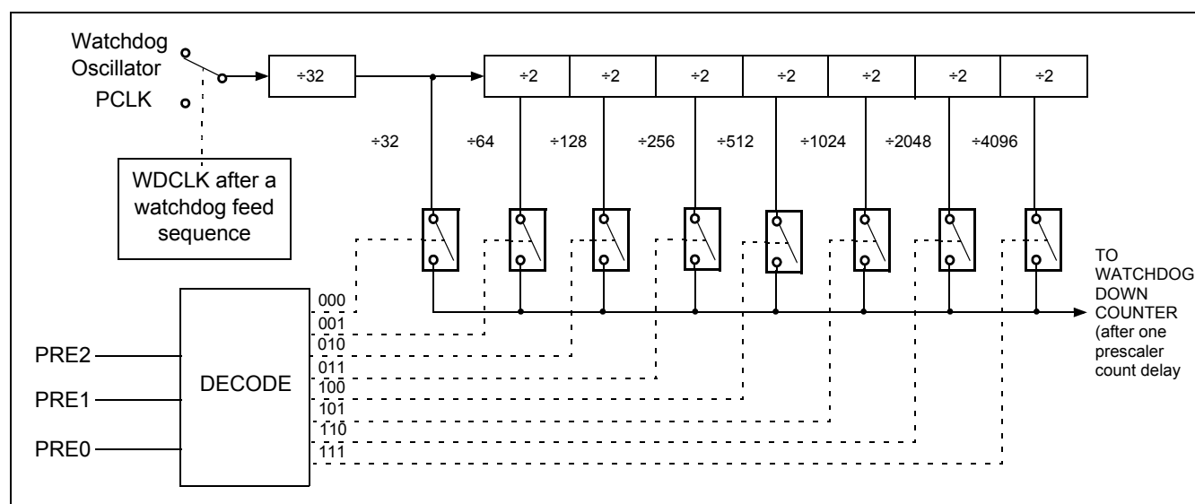
Figure 13-1: Watchdog Prescaler
