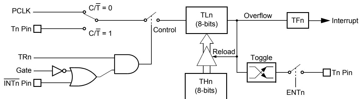
Figure 7-6: Timer/Counter 0 or 1 in Mode 2 (8-bit auto-reload)
