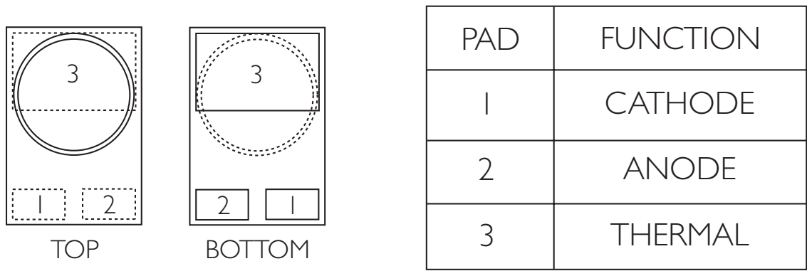
Figure 2. Pad configuration.
