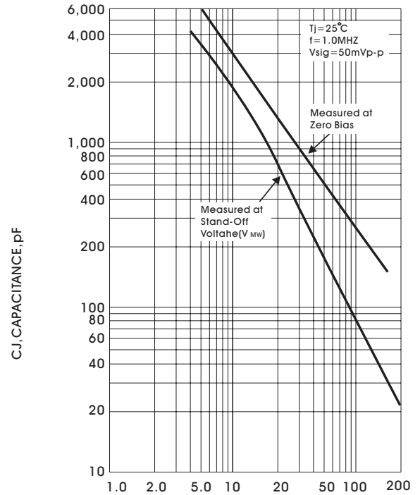
FIGURE 4 TYPICAL CAPACITANCE
