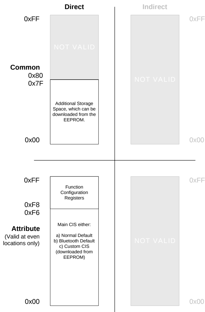
Figure 5: Normal Mode memory space map
