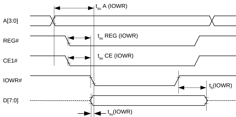
Figure 11: I/O write timing
