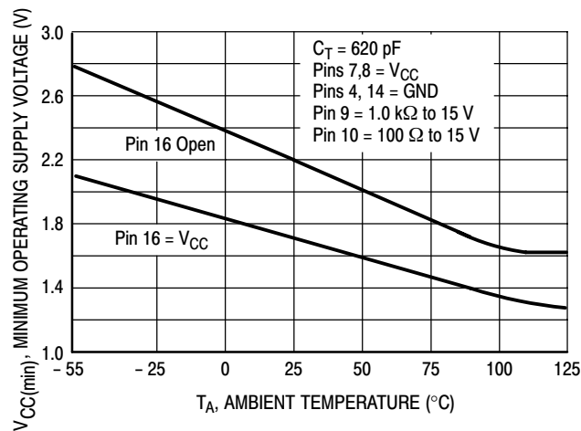
Figure 18. Minimum Operating Supply Voltage vs. Temperature
