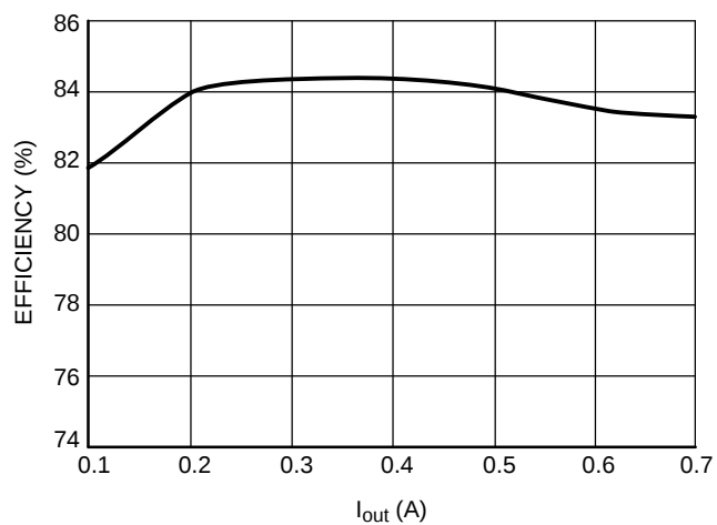
Figure 28. Efficiency vs. Output Current for the Boost Demo Board at V_{in} = 12 V, T_A = 25^\circ\text{C}
