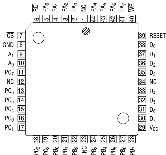
44 pin Plastic QFJ
