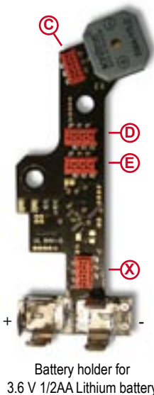
Hugyfot leakage detector with integrated strobe connections Nikon or Canon
