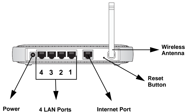
Figure 1-2: WGR614 v6 Rear Panel
