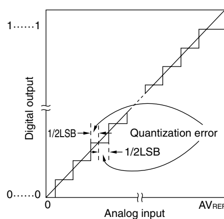
Figure 12-16. Quantization Error
