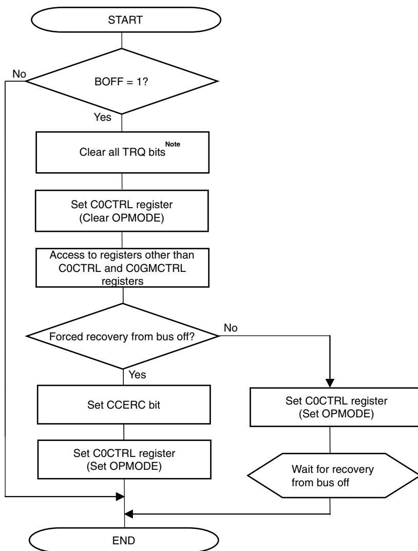
Figure 15-56. Bus-Off Recovery (Expect Normal Operation Mode with ABT)
