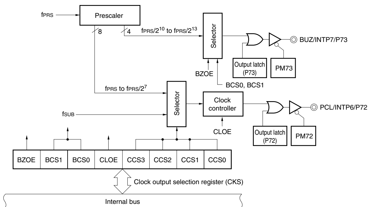
Figure 11-1. Block Diagram of Clock Output/Buzzer Output Controller
