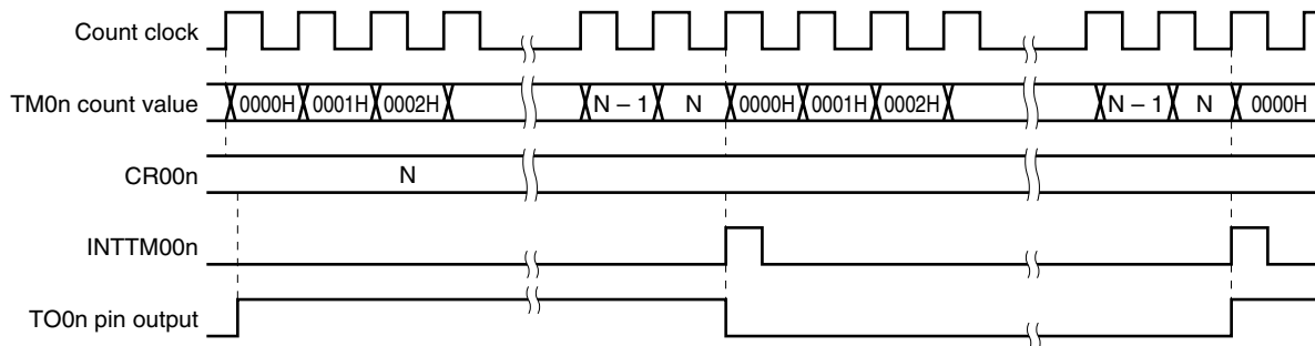
Figure 6-37. Square-Wave Output Operation Timing
