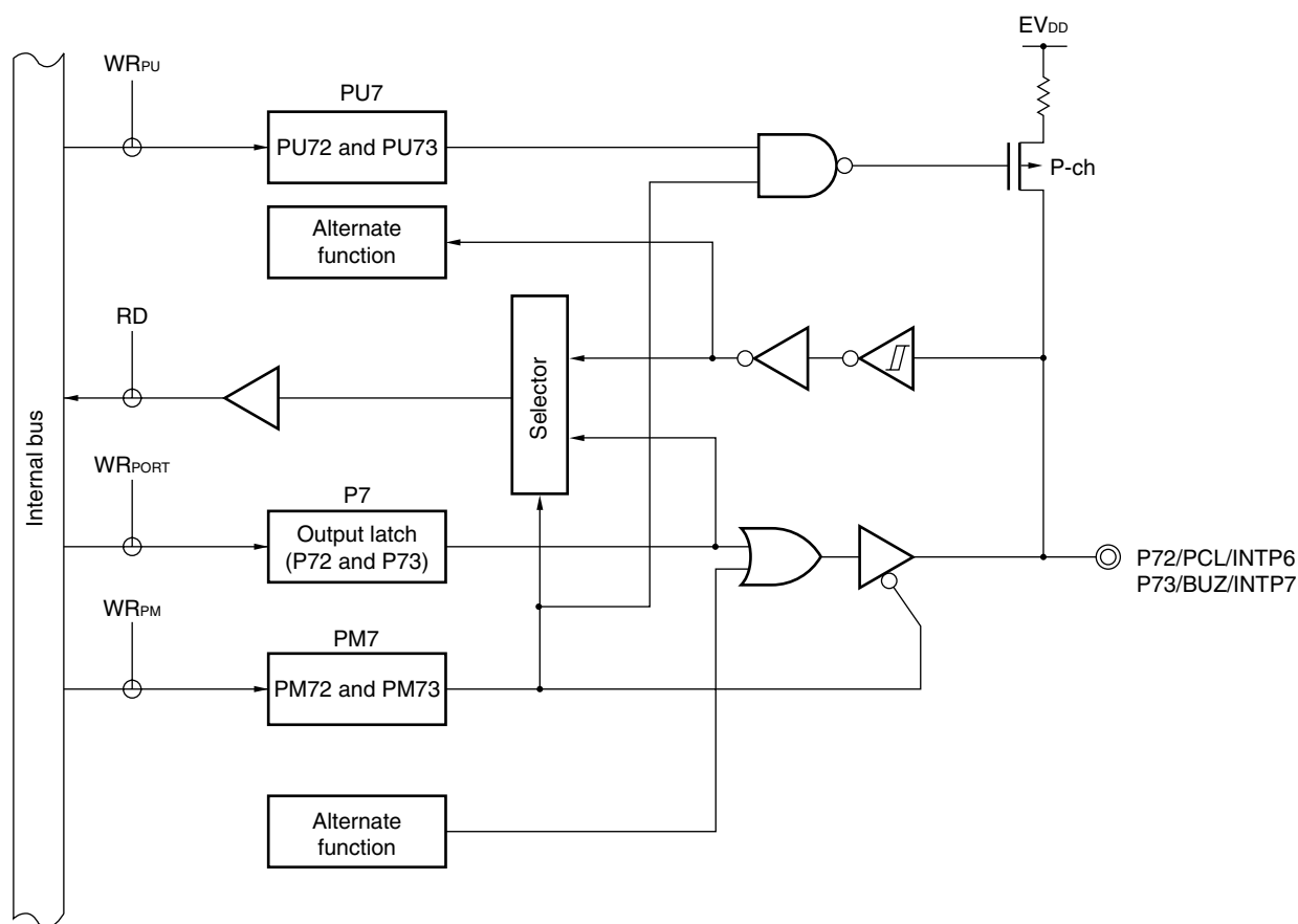
Figure 4-14. Block Diagram of P72 and P73
