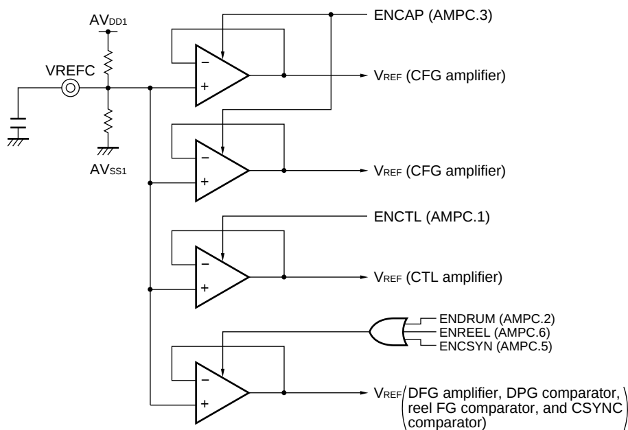
Figure 3-27. Block Diagram of Reference Amplifier
