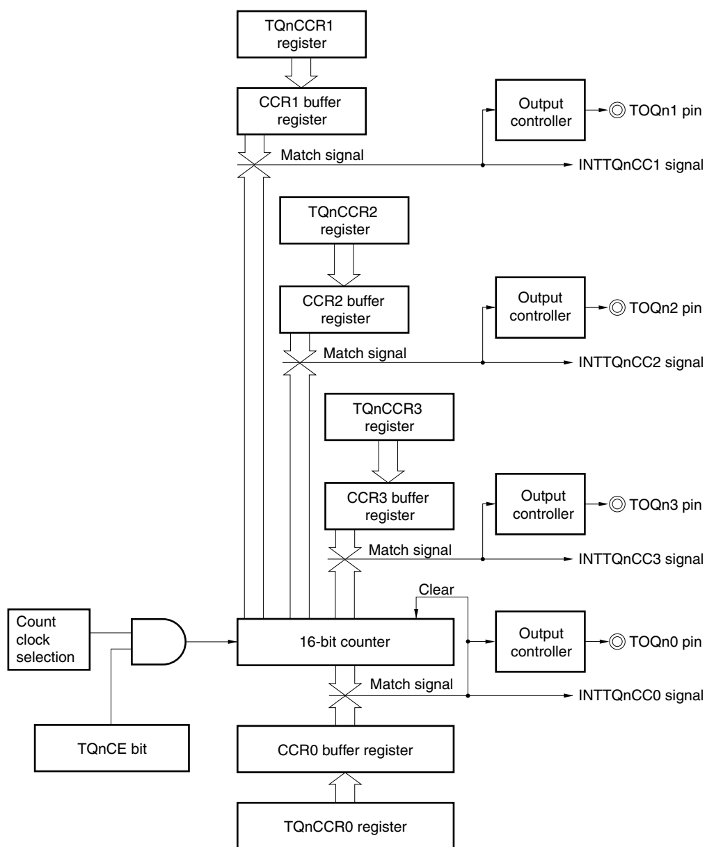
Figure 8-6. Configuration of TQnCCR1 to TQnCCR3 Registers
