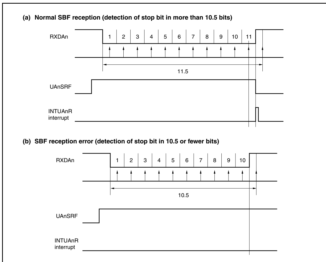
Figure 13-6. SBF Reception
