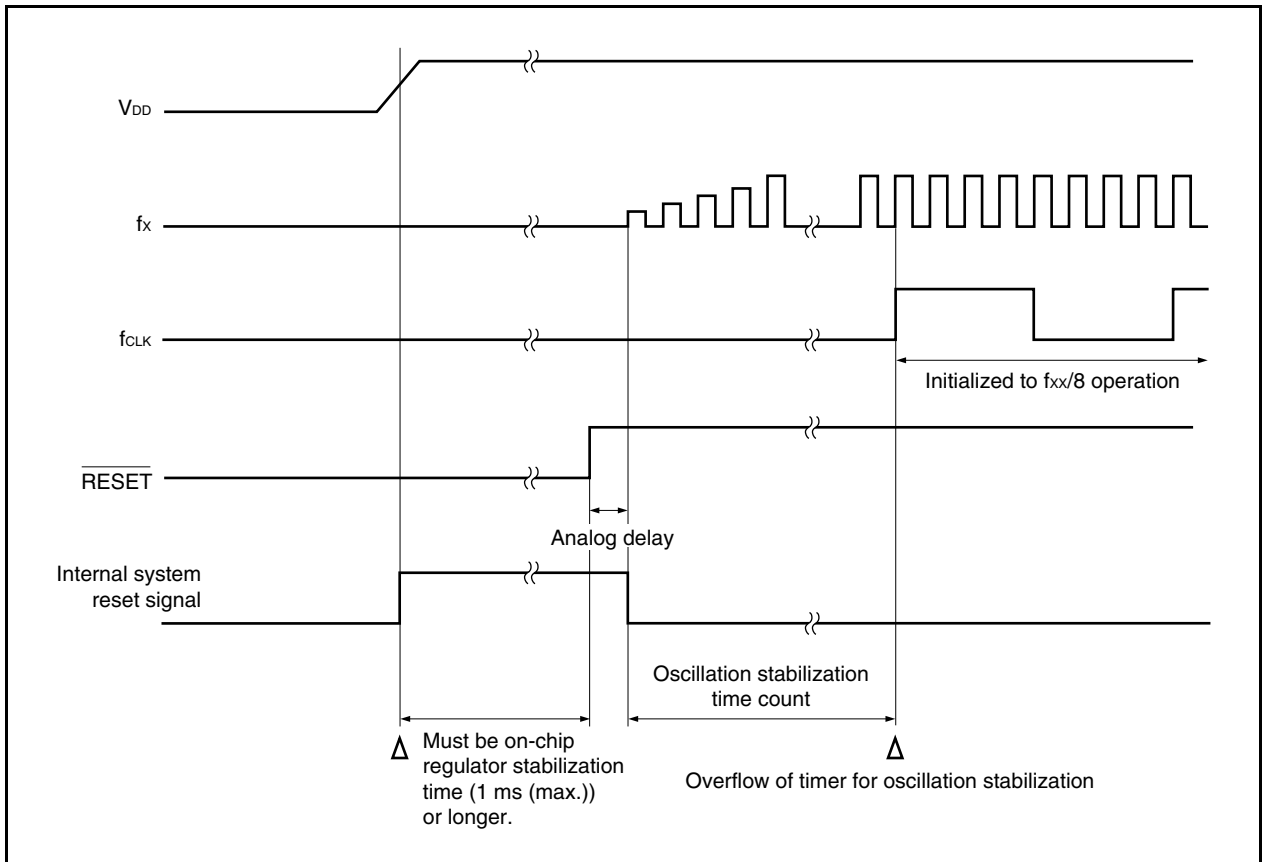
Figure 19-2. Timing of Power-on Reset Operation
