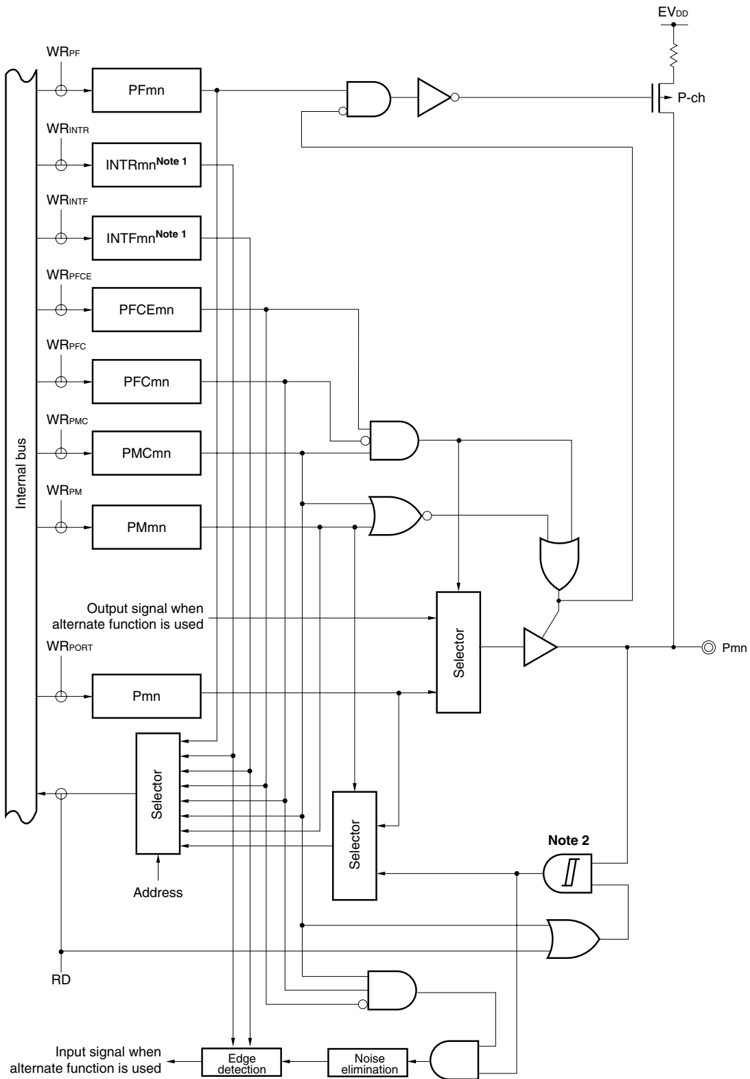
Figure 4-29. Block Diagram of Type W-1
