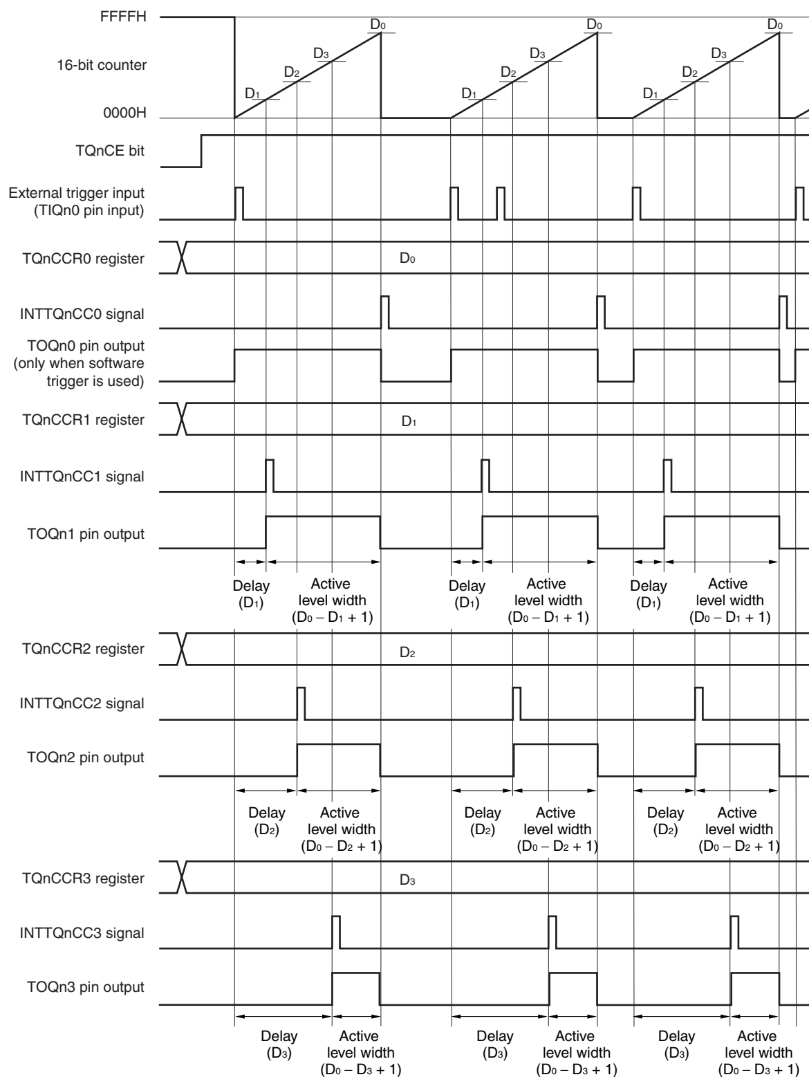
Figure 8-21. Basic Timing in One-Shot Pulse Output Mode
