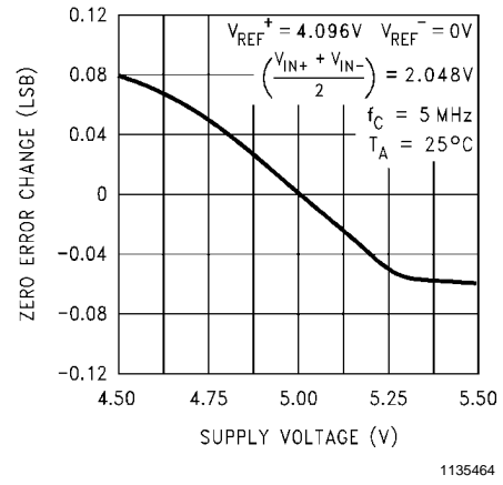
Offset or Zero Error Change vs. Supply Voltage
