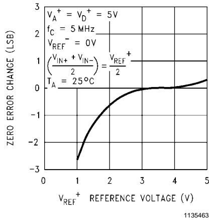
Offset or Zero Error Change vs. Reference Voltage
