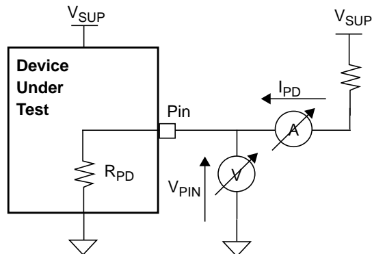
Figure 14. Internal Resistor Test Conditions, T_A = 0^\circ\text{C} to 70^\circ\text{C} , V_{SUP} = 3.3\text{V}
