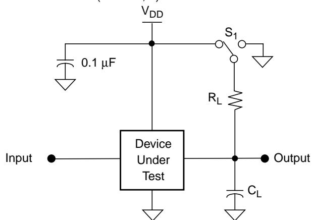
Figure 16. AC Test Conditions, T_A = 0^\circ\text{C} to 70^\circ\text{C} , V_{DD} = 3.3\text{V} \pm 10\%
