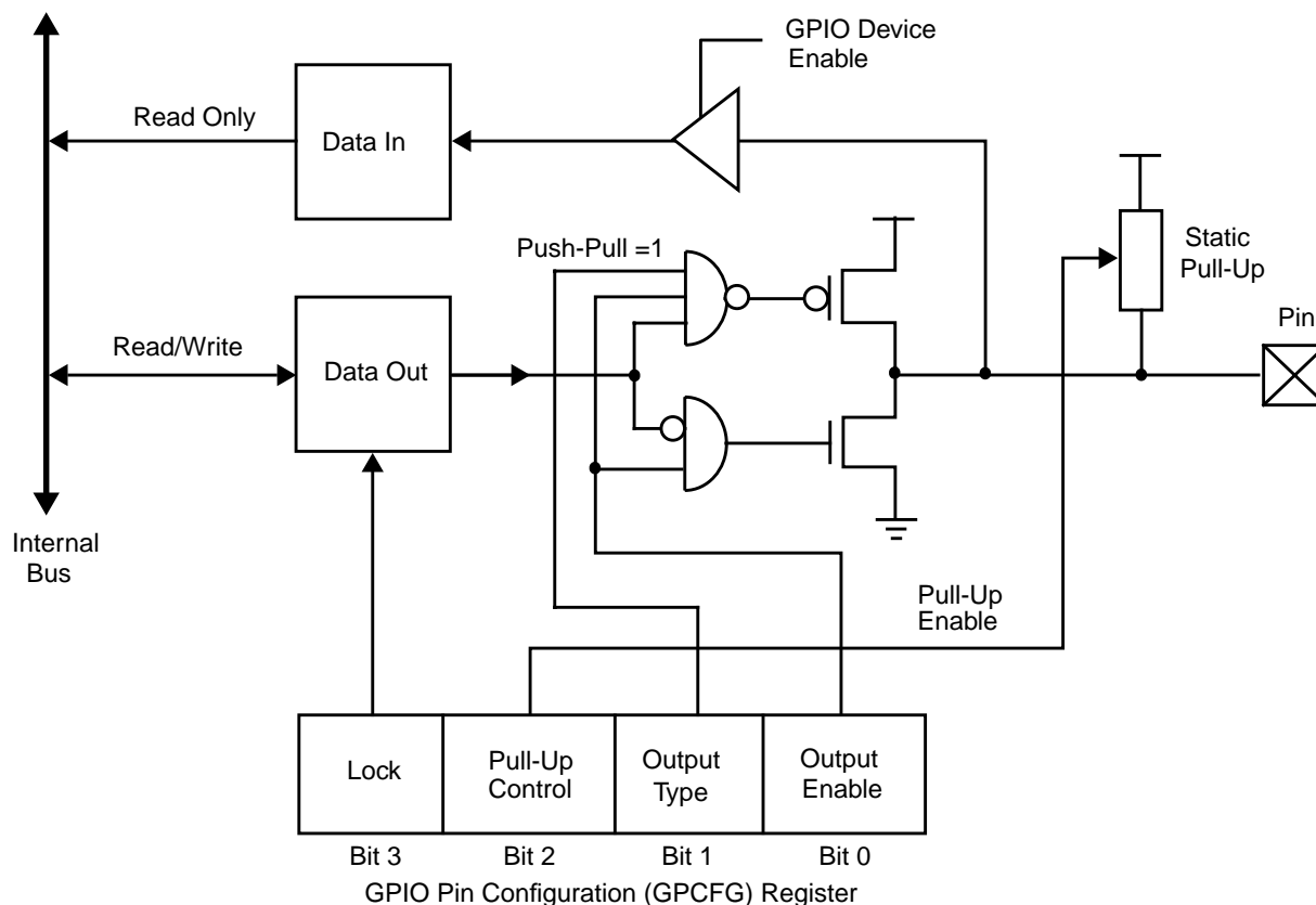
Figure 9. GPIO Basic Functionality
