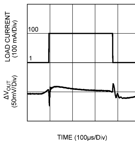
Load Transient
