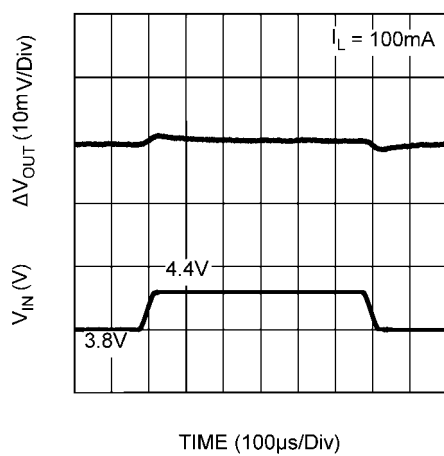
Line Transient
