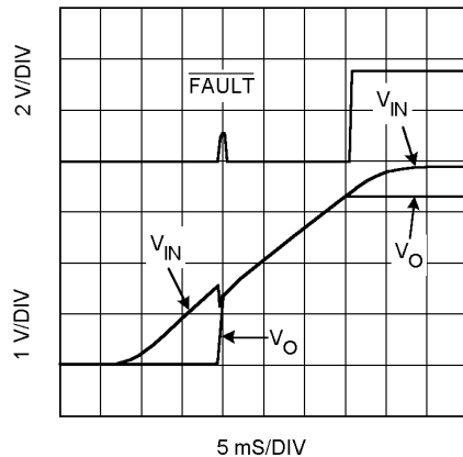
Power-Up Response
