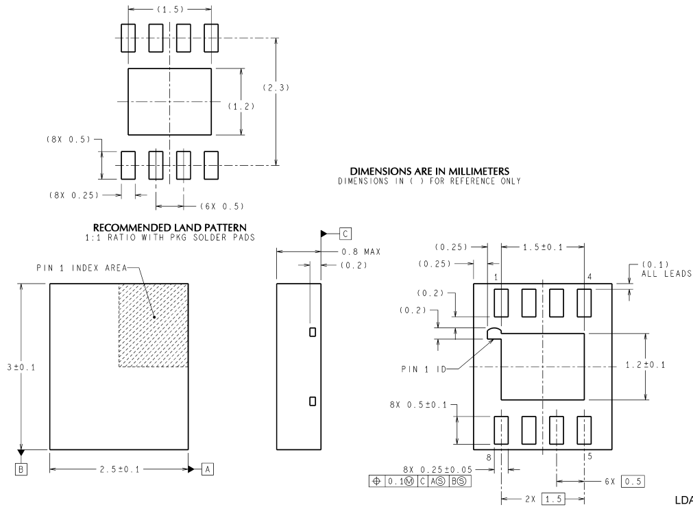
8-Lead LLP Surface Mount NS Package Number LDA08C
