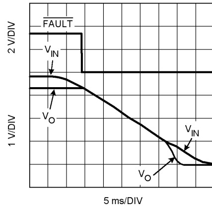
Power-Down Response
