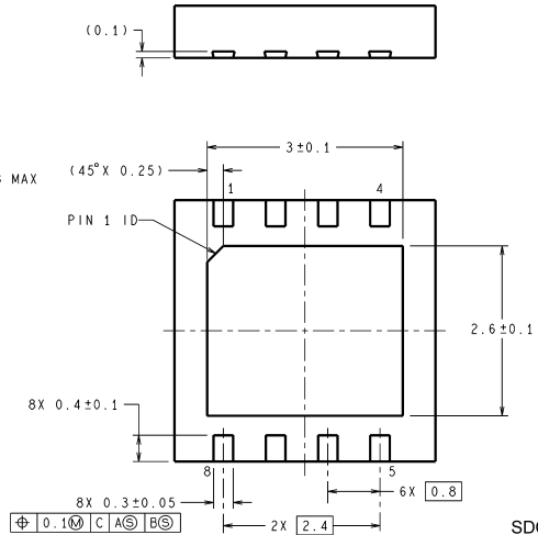
8 Lead LLP Surface Mount Package NS Package Number SDC08A
