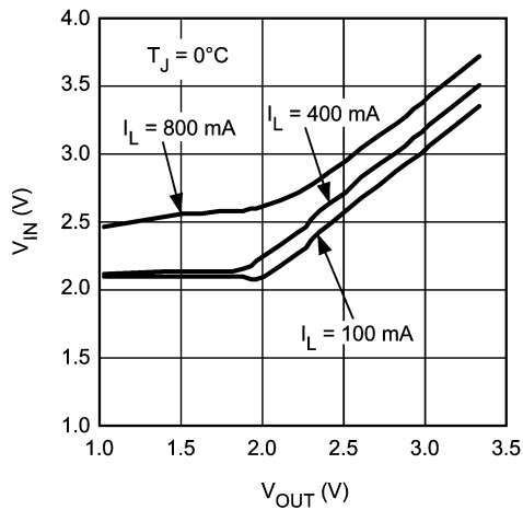
Minimum V_{IN} vs V_{OUT}
