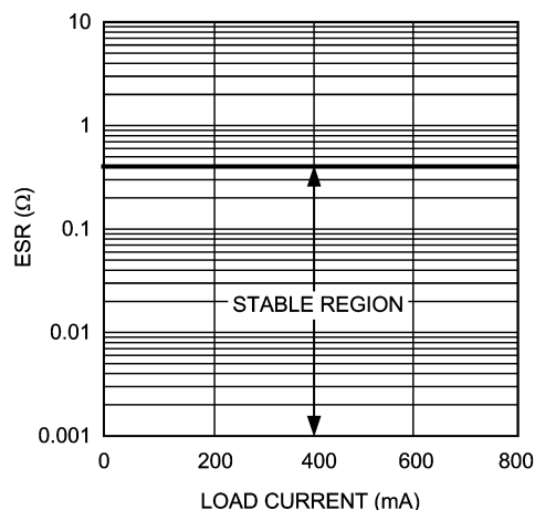
FIGURE 1. Stable Region For Output Capacitor ESR
