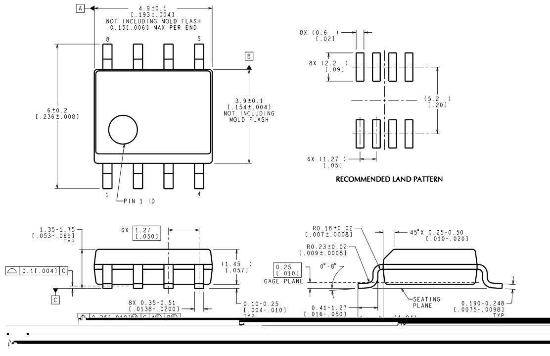
SO-8 Package NS Package Number M08A
