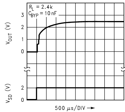
Turn-ON Waveform
