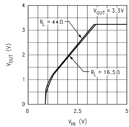
Dropout Characteristics
