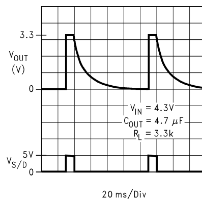
Turn-Off Waveform
