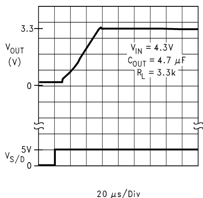
Turn-On Waveform
